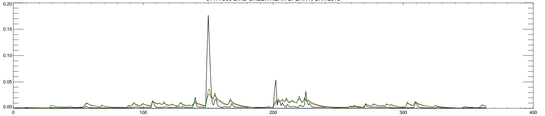
07177500 BIRD CREEK NEAR SPERRY, OK : 2014
