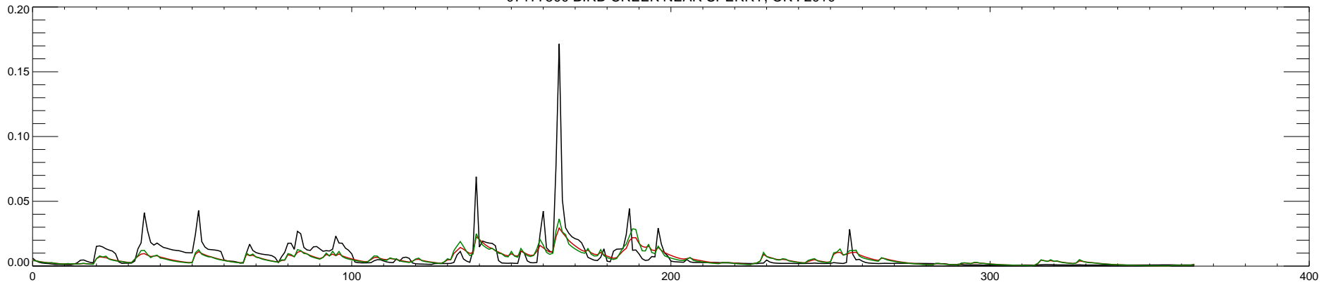
07177500 BIRD CREEK NEAR SPERRY, OK : 2011
