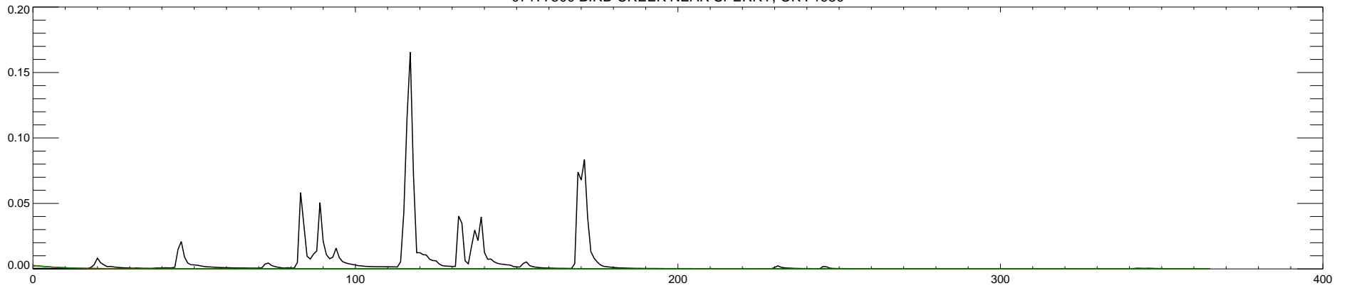
07177500 BIRD CREEK NEAR SPERRY, OK : 1981
