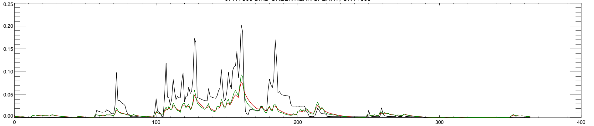
07177500 BIRD CREEK NEAR SPERRY, OK : 1996
