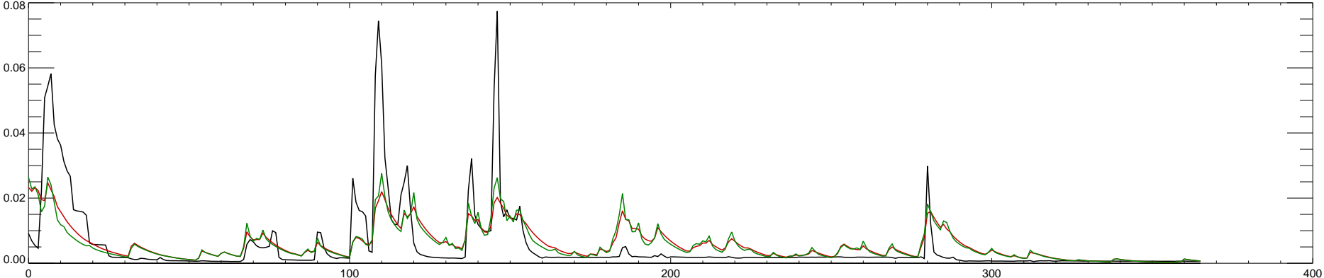
07177500 BIRD CREEK NEAR SPERRY, OK : 2016
