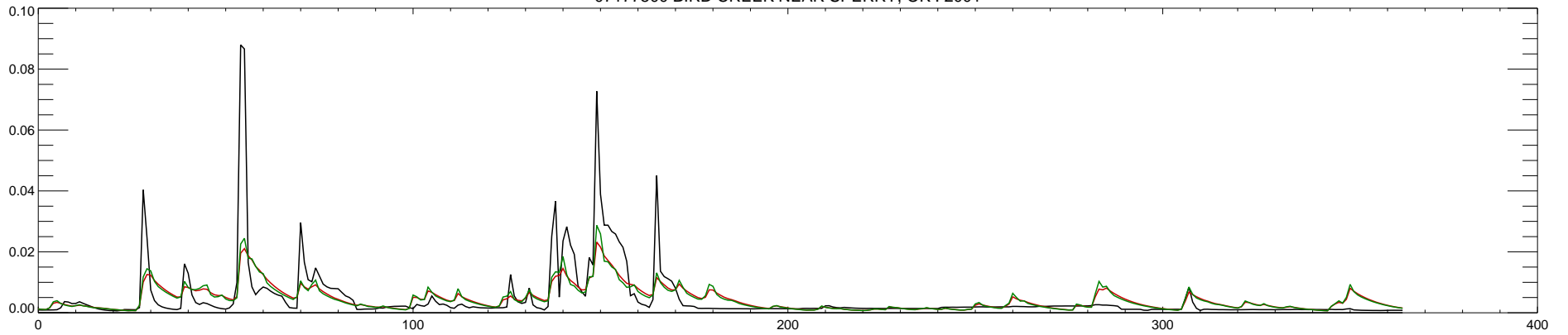
07177500 BIRD CREEK NEAR SPERRY, OK : 2002
