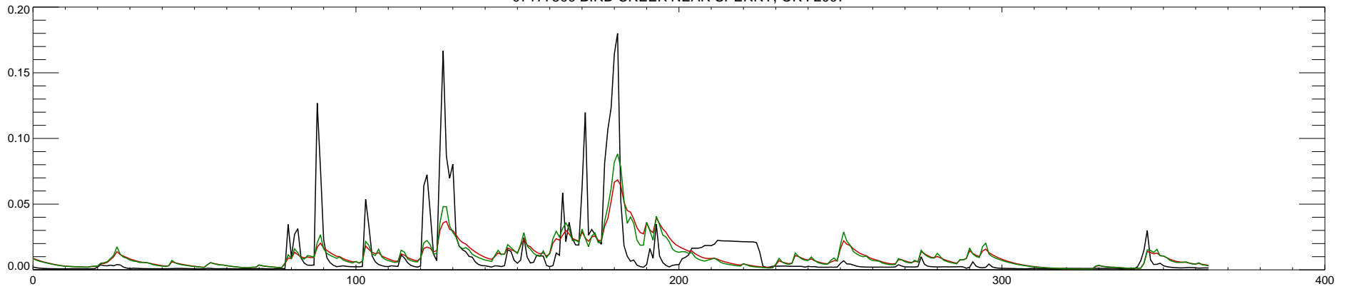
07177500 BIRD CREEK NEAR SPERRY, OK : 2008
