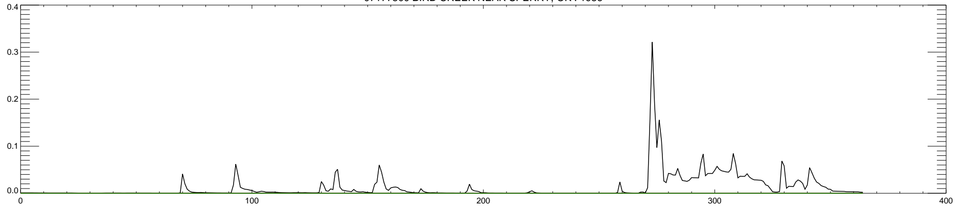
07177500 BIRD CREEK NEAR SPERRY, OK : 1987
