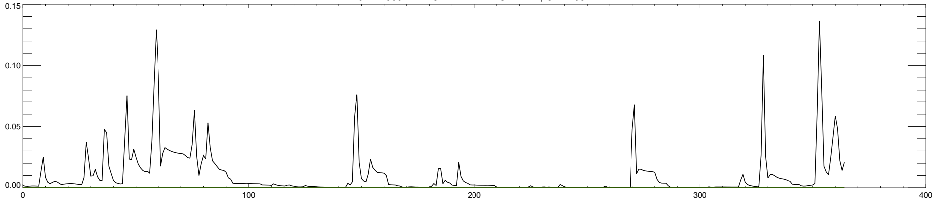
07177500 BIRD CREEK NEAR SPERRY, OK : 1988
