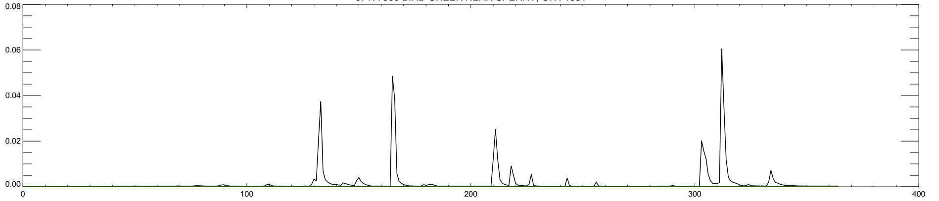
07177500 BIRD CREEK NEAR SPERRY, OK : 1982
