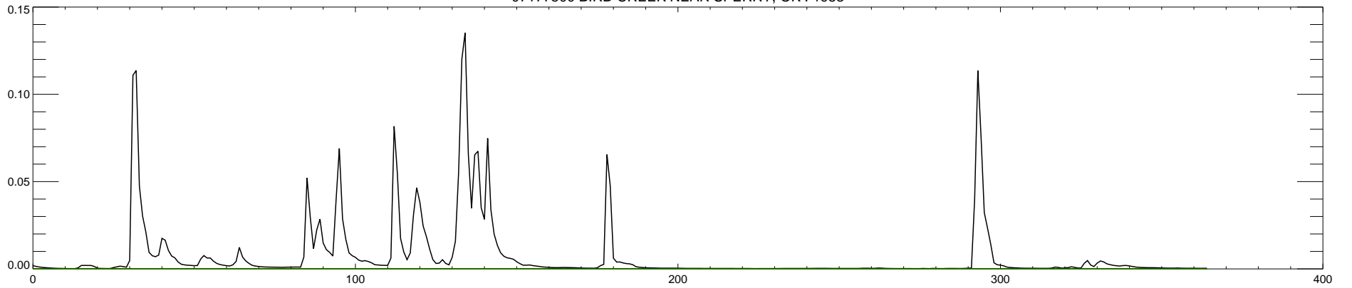
07177500 BIRD CREEK NEAR SPERRY, OK : 1984
