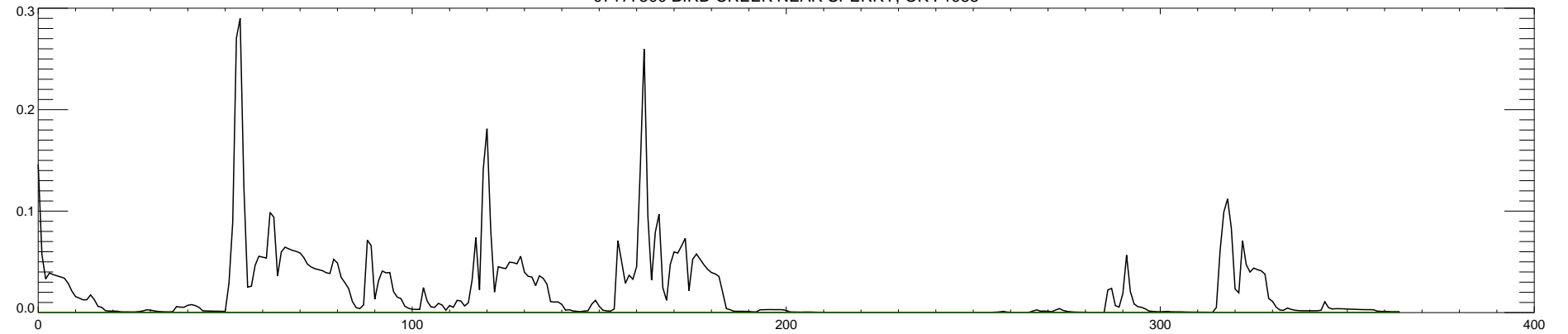
07177500 BIRD CREEK NEAR SPERRY, OK : 1985
