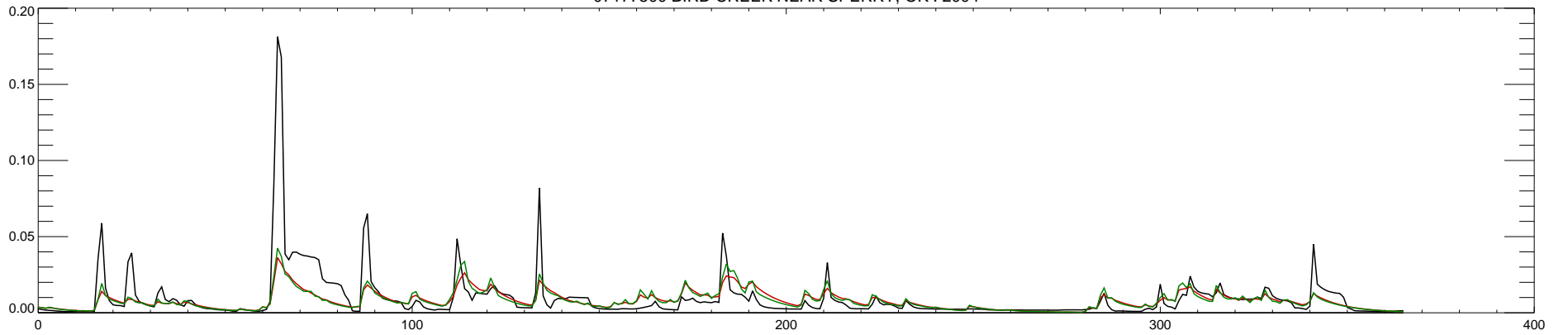
07177500 BIRD CREEK NEAR SPERRY, OK : 2005
