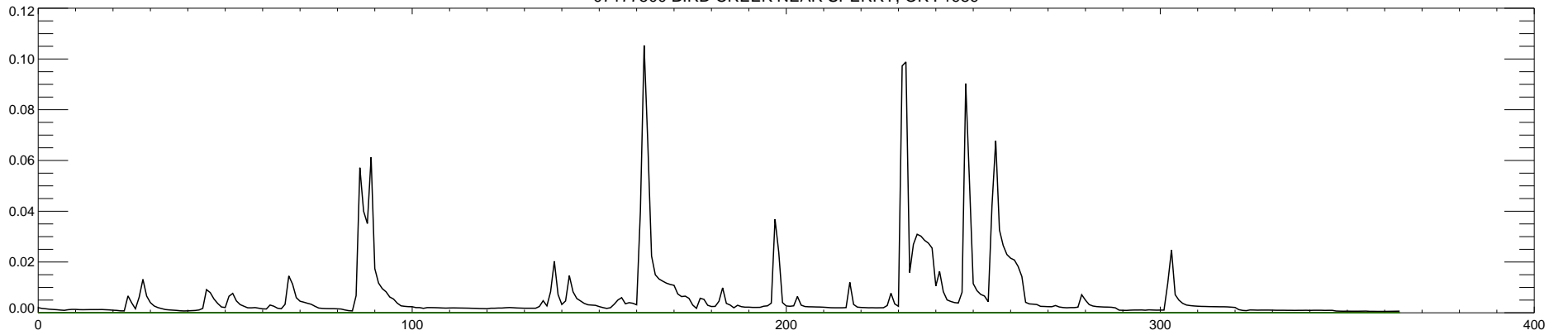
07177500 BIRD CREEK NEAR SPERRY, OK : 1990
