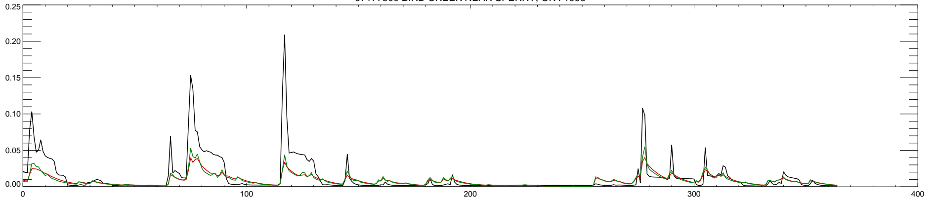
07177500 BIRD CREEK NEAR SPERRY, OK : 1999
