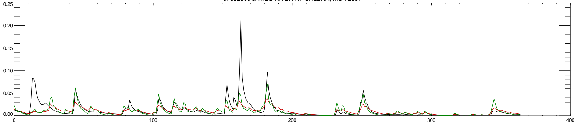
07052500 JAMES RIVER AT GALENA, MO : 2008
