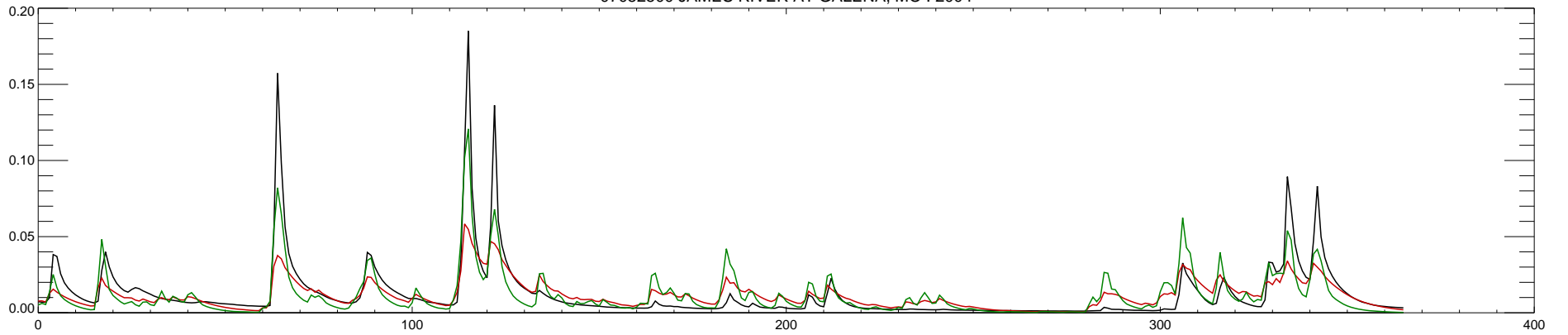
07052500 JAMES RIVER AT GALENA, MO : 2005
