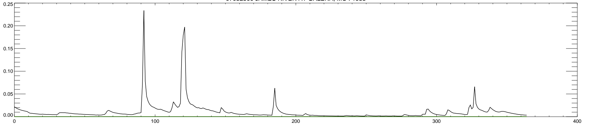
07052500 JAMES RIVER AT GALENA, MO : 1984
