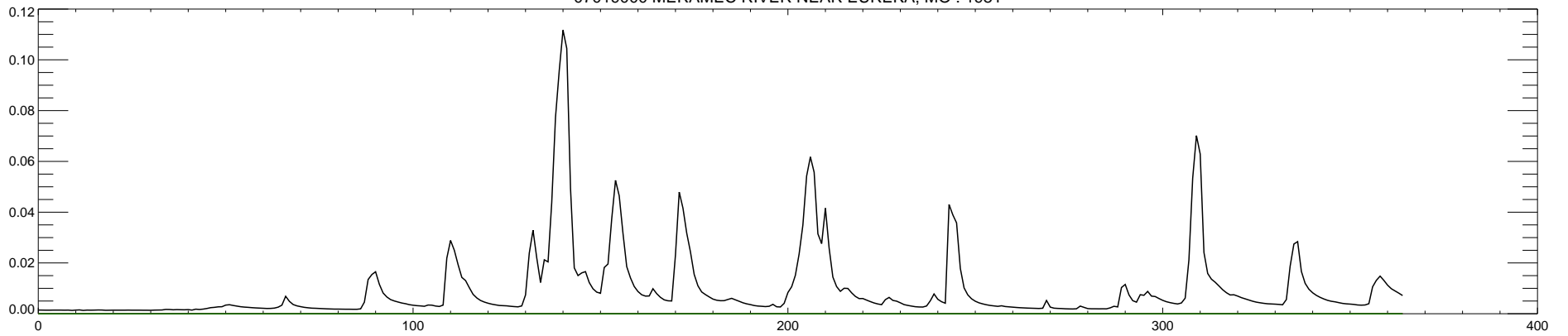
07019000 MERAMEC RIVER NEAR EUREKA, MO : 1982
