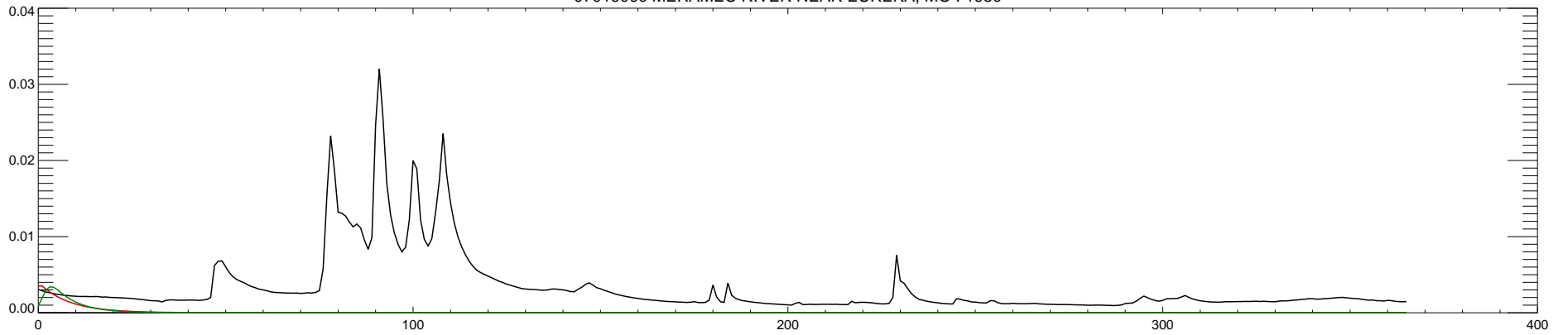
07019000 MERAMEC RIVER NEAR EUREKA, MO : 1981
