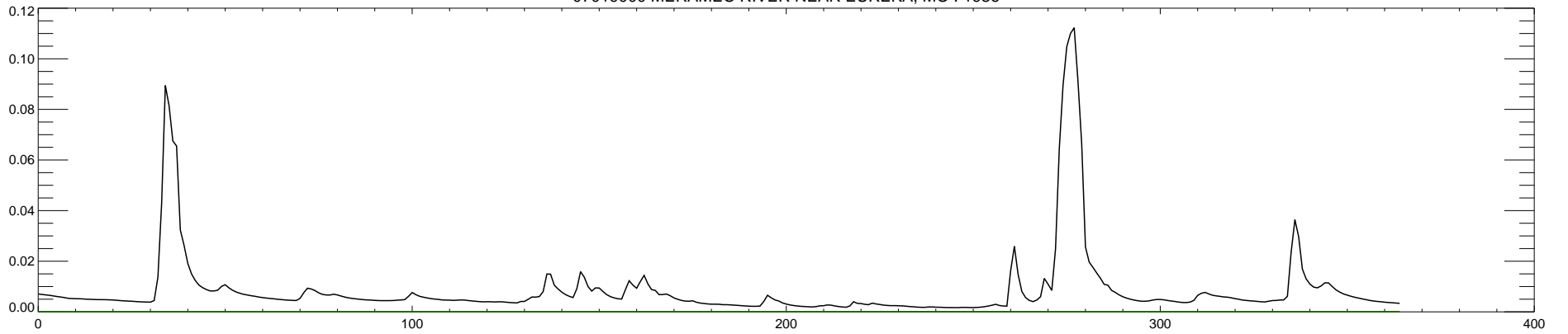
07019000 MERAMEC RIVER NEAR EUREKA, MO : 1987
