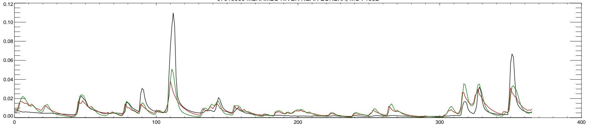
07019000 MERAMEC RIVER NEAR EUREKA, MO : 1993
