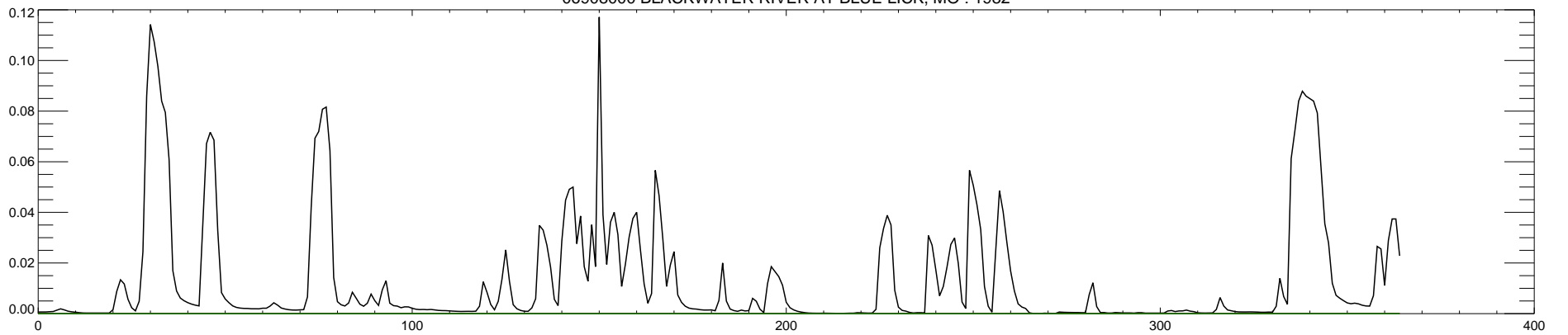
06908000 BLACKWATER RIVER AT BLUE LICK, MO : 1982
