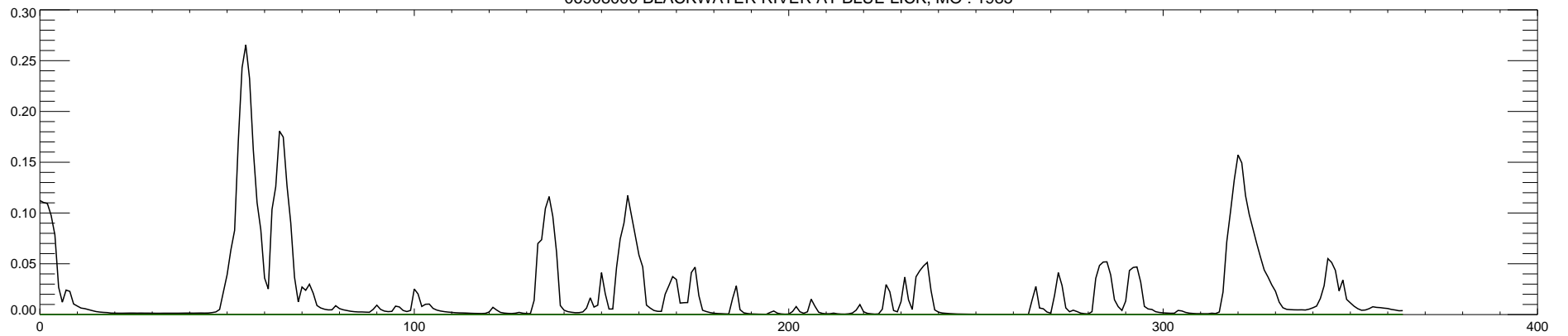
06908000 BLACKWATER RIVER AT BLUE LICK, MO : 1985
