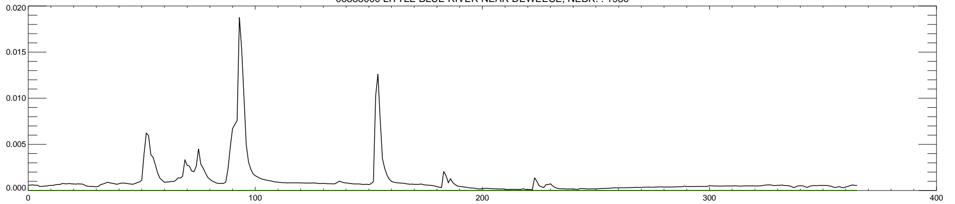
06883000 LITTLE BLUE RIVER NEAR DEWEESE, NEBR. : 1981
