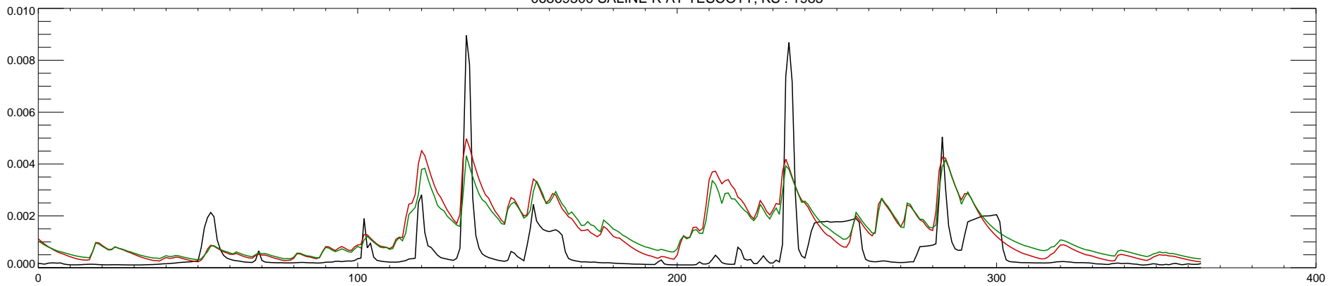
06869500 SALINE R AT TESCOTT, KS : 1985
