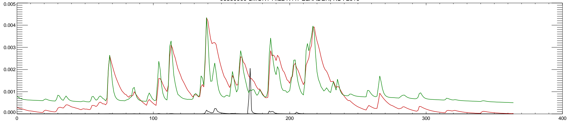
06860000 SMOKY HILL R AT ELKADER, KS : 2011
