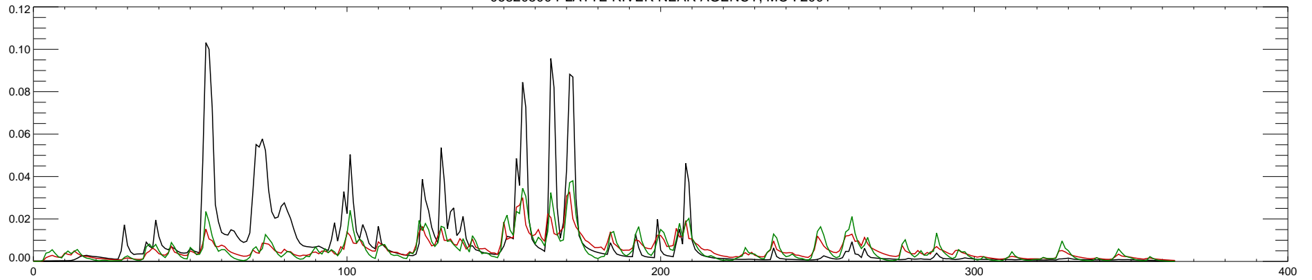
06820500 PLATTE RIVER NEAR AGENCY, MO : 2002
