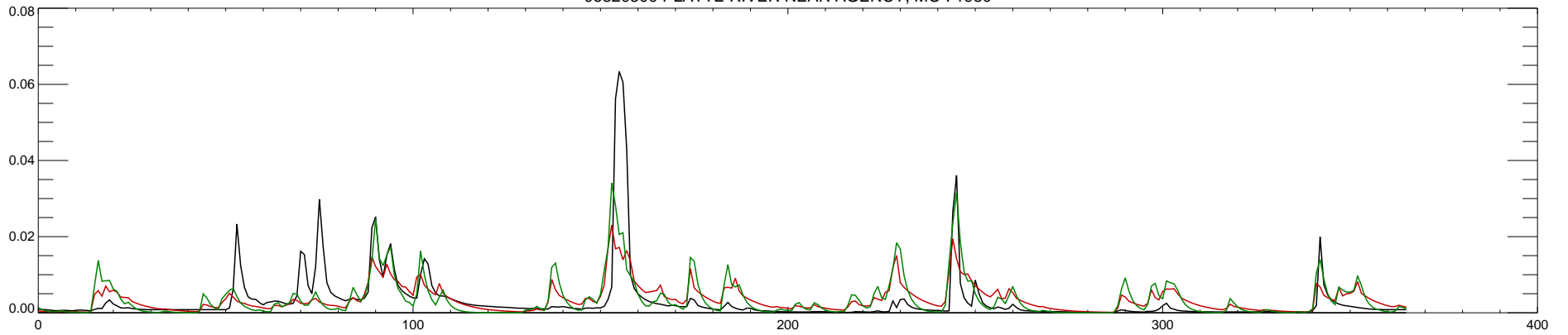
06820500 PLATTE RIVER NEAR AGENCY, MO : 1981
