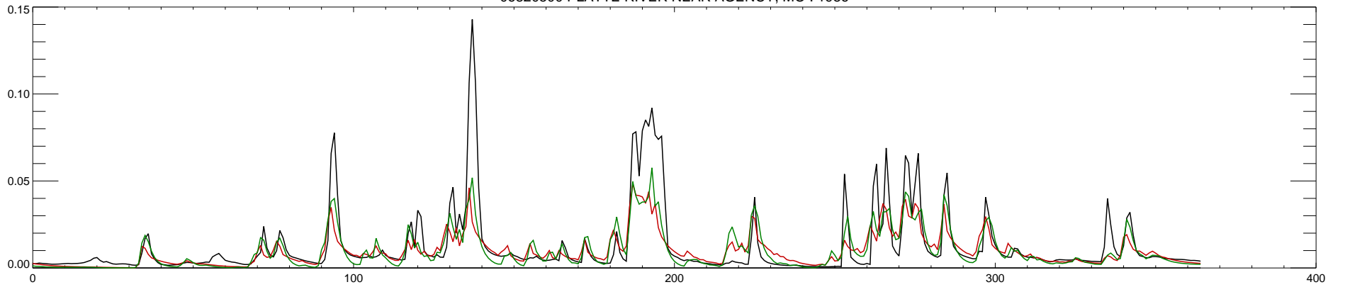
06820500 PLATTE RIVER NEAR AGENCY, MO : 1987
