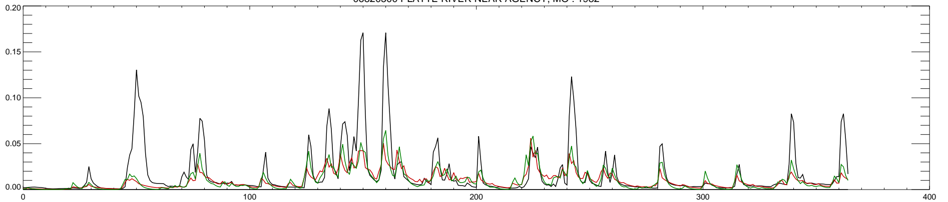
06820500 PLATTE RIVER NEAR AGENCY, MO : 1982
