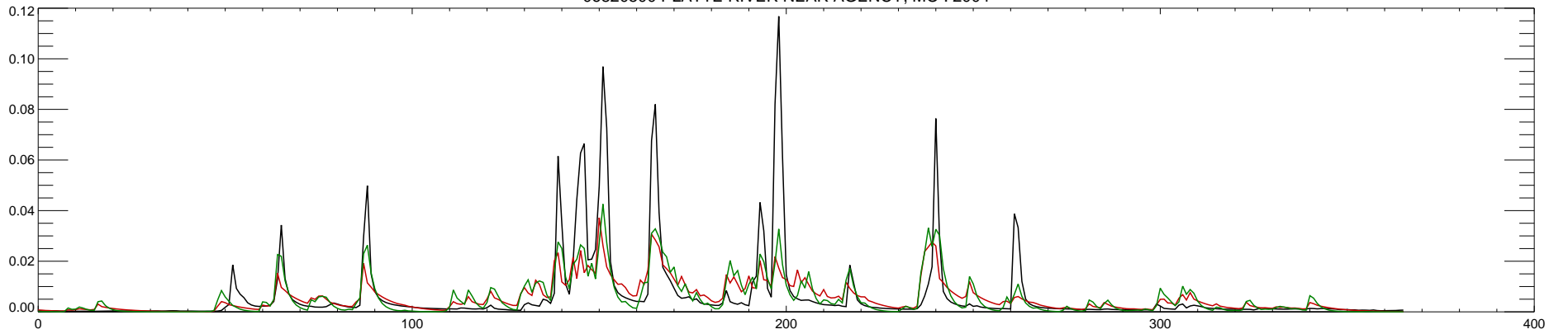
06820500 PLATTE RIVER NEAR AGENCY, MO : 2005
