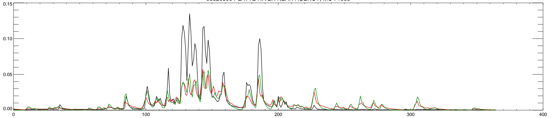
06820500 PLATTE RIVER NEAR AGENCY, MO : 1996
