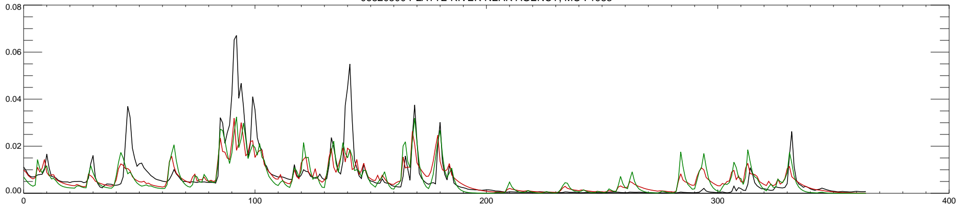
06820500 PLATTE RIVER NEAR AGENCY, MO : 1984
