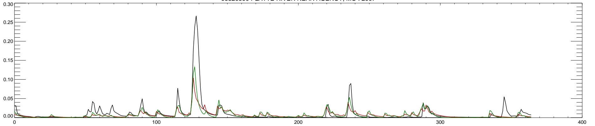
06820500 PLATTE RIVER NEAR AGENCY, MO : 2008
