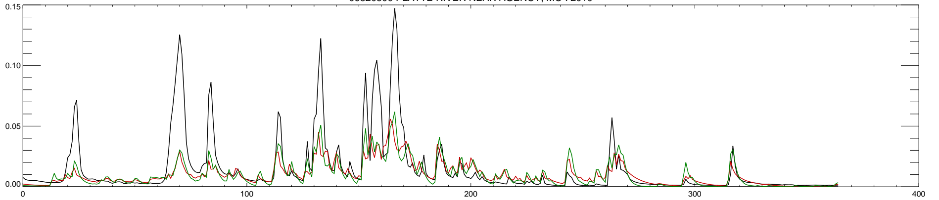
06820500 PLATTE RIVER NEAR AGENCY, MO : 2011
