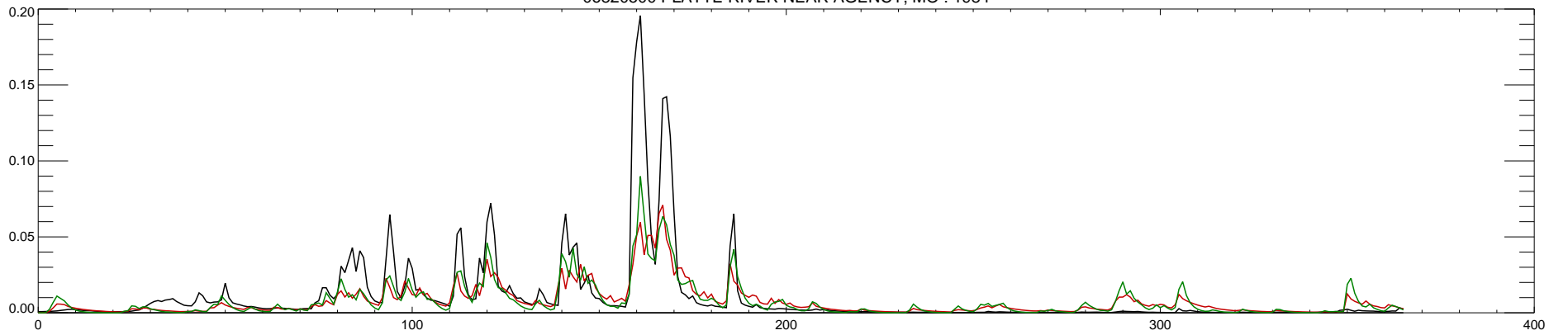
06820500 PLATTE RIVER NEAR AGENCY, MO : 1985
