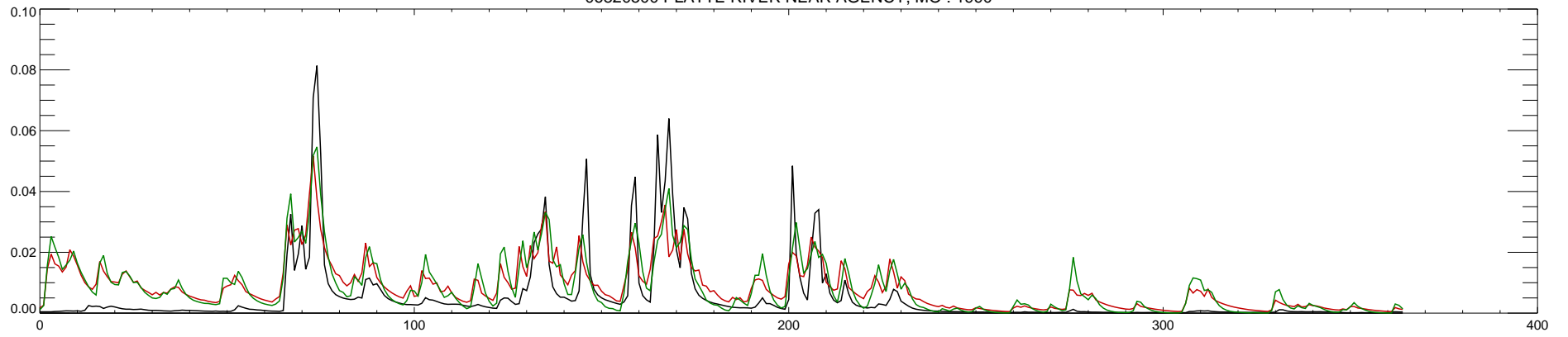
06820500 PLATTE RIVER NEAR AGENCY, MO : 1991
