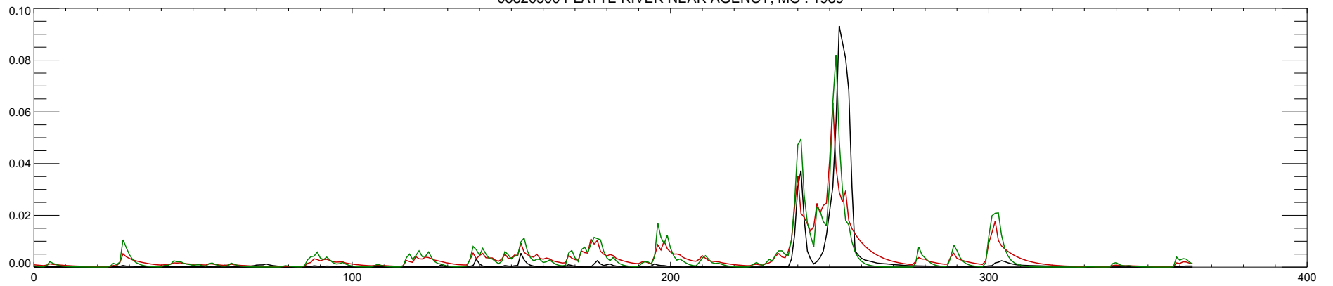
06820500 PLATTE RIVER NEAR AGENCY, MO : 1990
