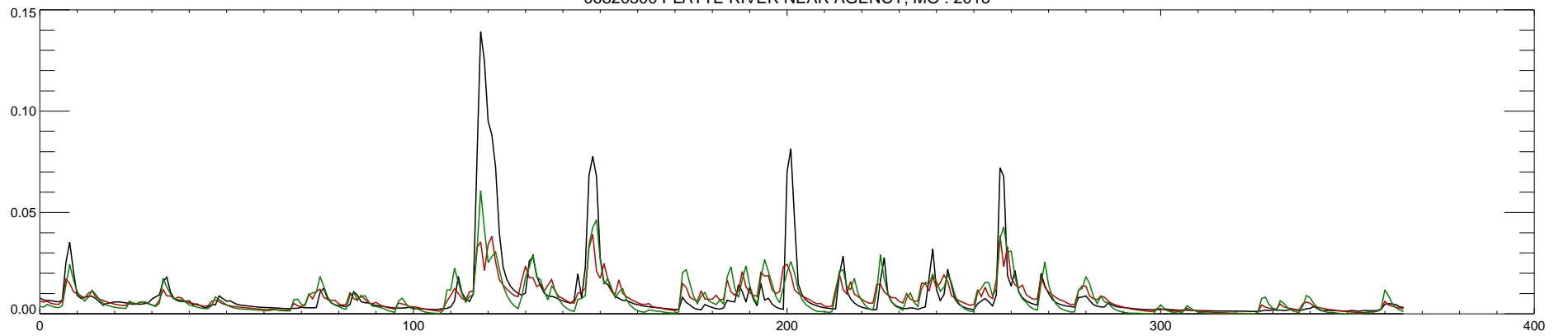
06820500 PLATTE RIVER NEAR AGENCY, MO : 2016
