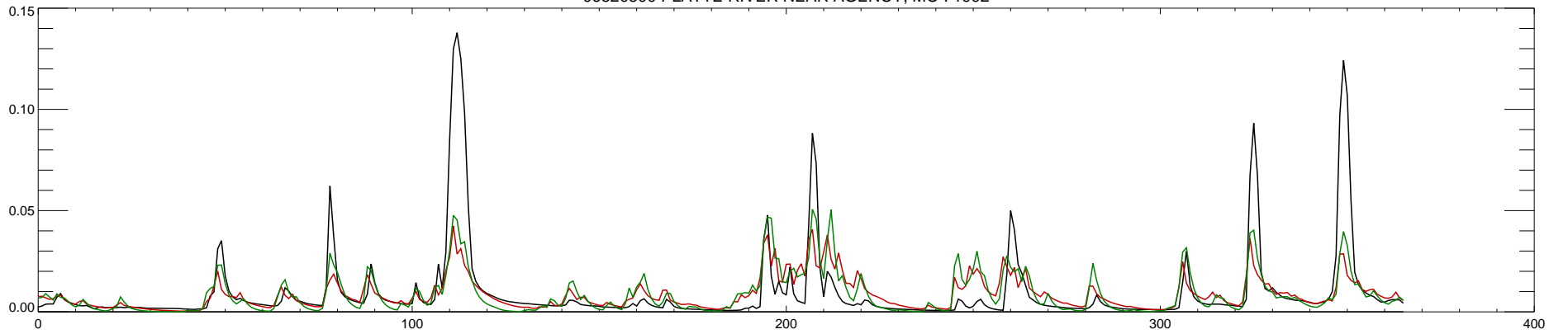
06820500 PLATTE RIVER NEAR AGENCY, MO : 1993
