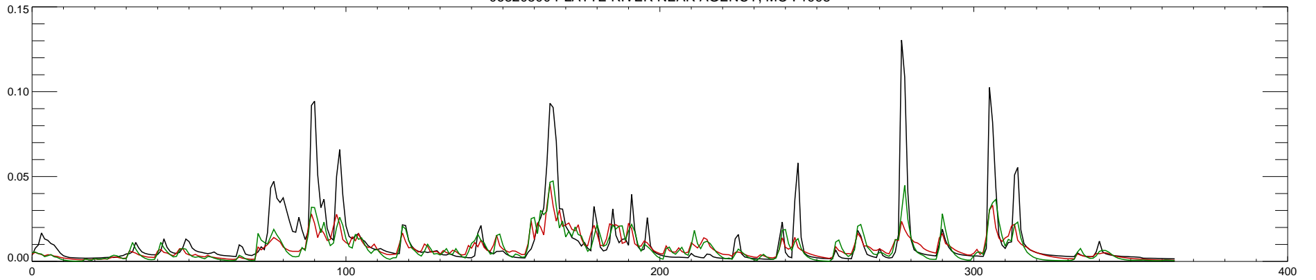
06820500 PLATTE RIVER NEAR AGENCY, MO : 1999
