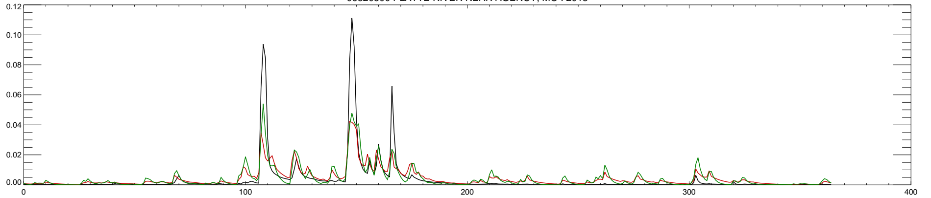
06820500 PLATTE RIVER NEAR AGENCY, MO : 2014
