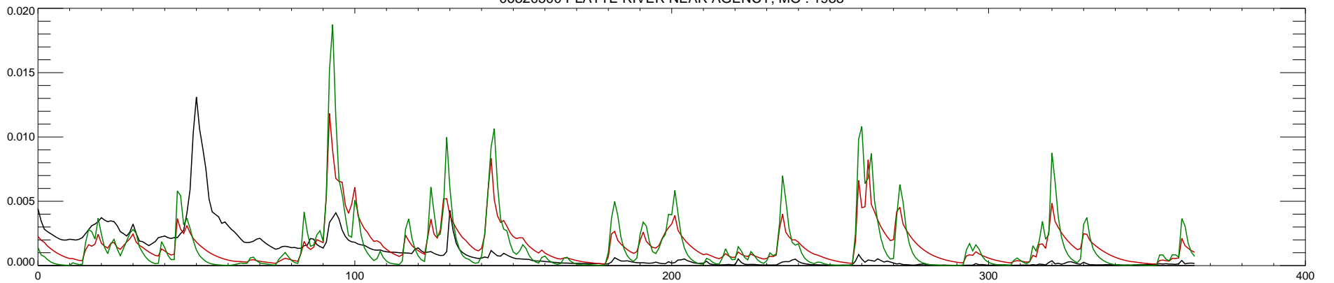
06820500 PLATTE RIVER NEAR AGENCY, MO : 1988
