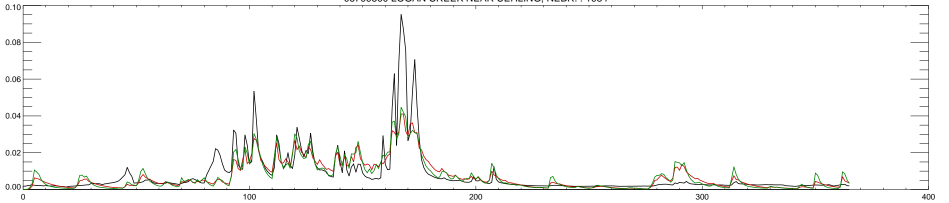
06799500 LOGAN CREEK NEAR UEHLING, NEBR. : 1985
