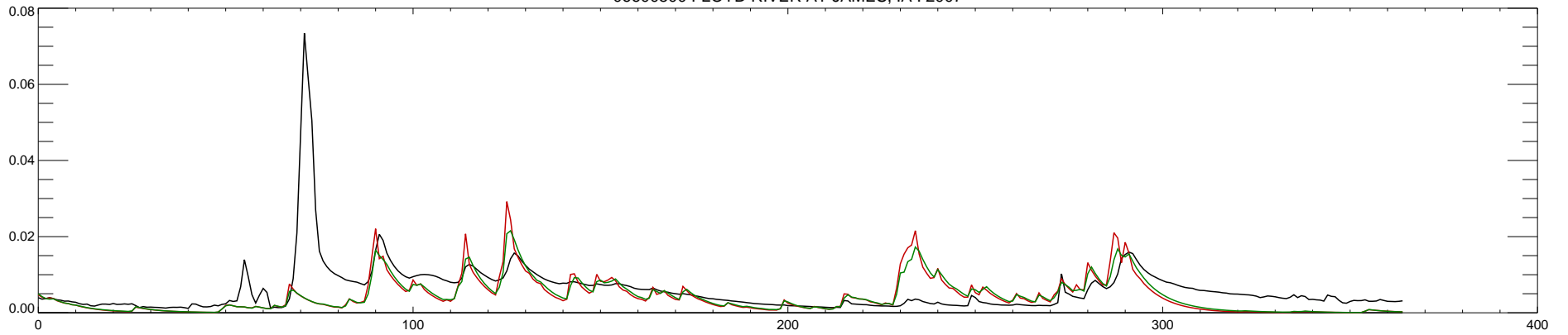
06600500 FLOYD RIVER AT JAMES, IA : 2008
