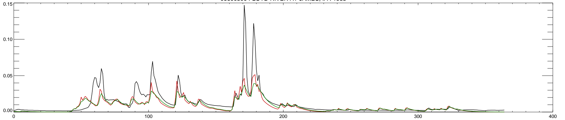
06600500 FLOYD RIVER AT JAMES, IA : 1984
