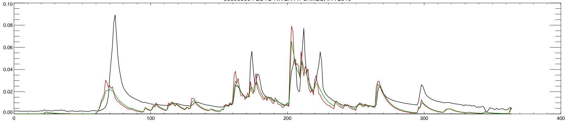
06600500 FLOYD RIVER AT JAMES, IA : 2011
