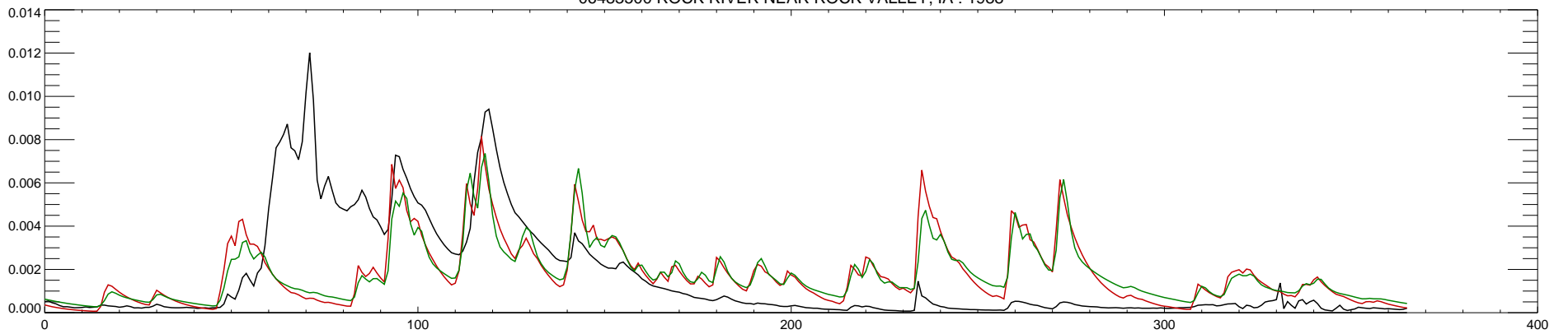
06483500 ROCK RIVER NEAR ROCK VALLEY, IA : 1988
