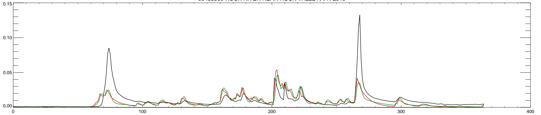
06483500 ROCK RIVER NEAR ROCK VALLEY, IA : 2011
