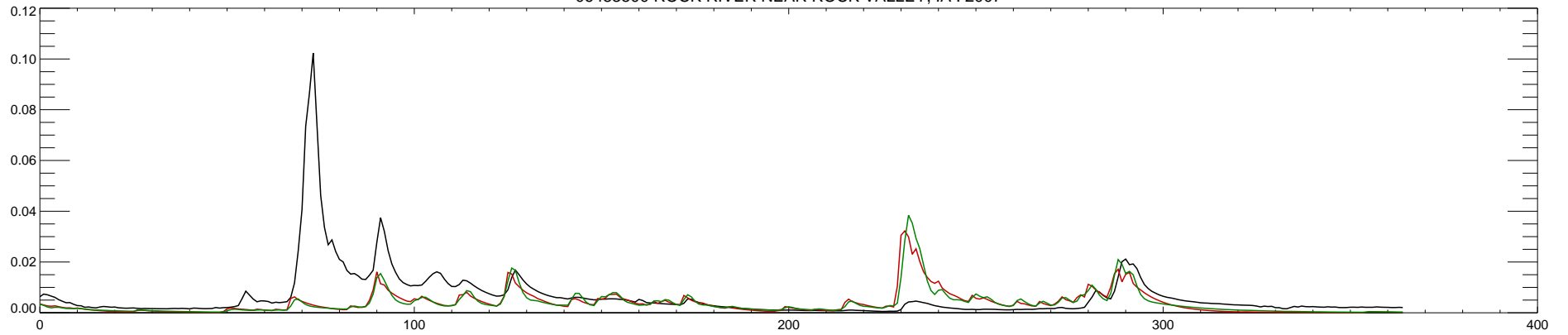
06483500 ROCK RIVER NEAR ROCK VALLEY, IA : 2008
