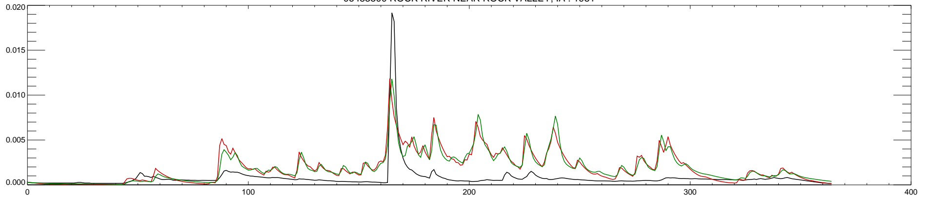
06483500 ROCK RIVER NEAR ROCK VALLEY, IA : 1982
