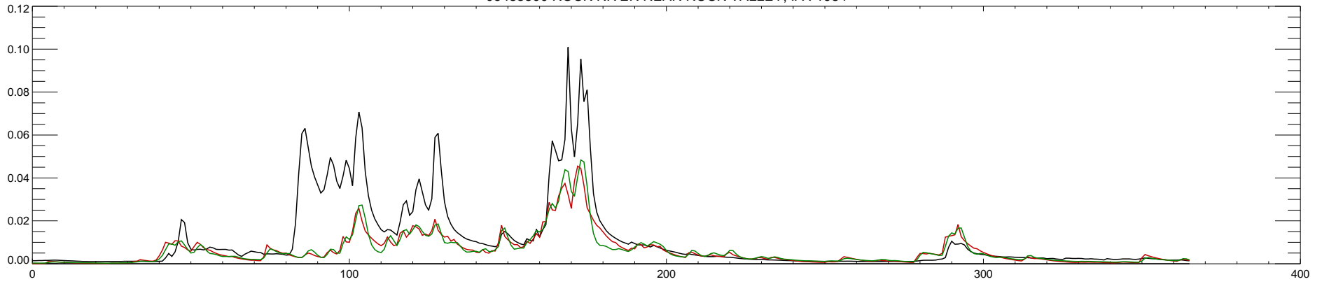
06483500 ROCK RIVER NEAR ROCK VALLEY, IA : 1985
