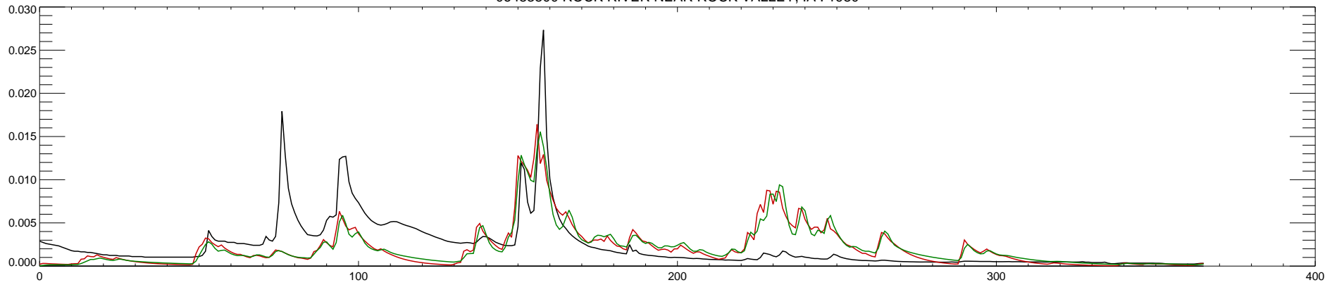
06483500 ROCK RIVER NEAR ROCK VALLEY, IA : 1981
