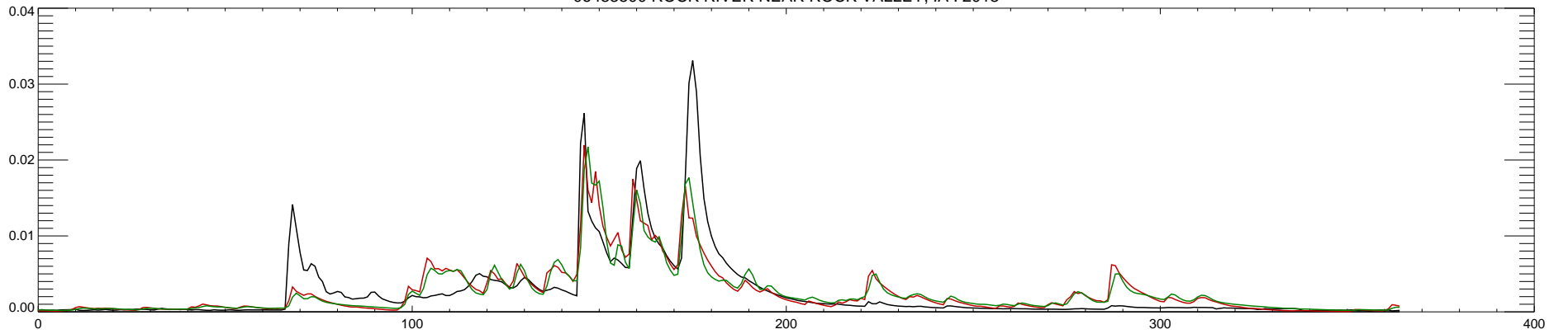
06483500 ROCK RIVER NEAR ROCK VALLEY, IA : 2014
