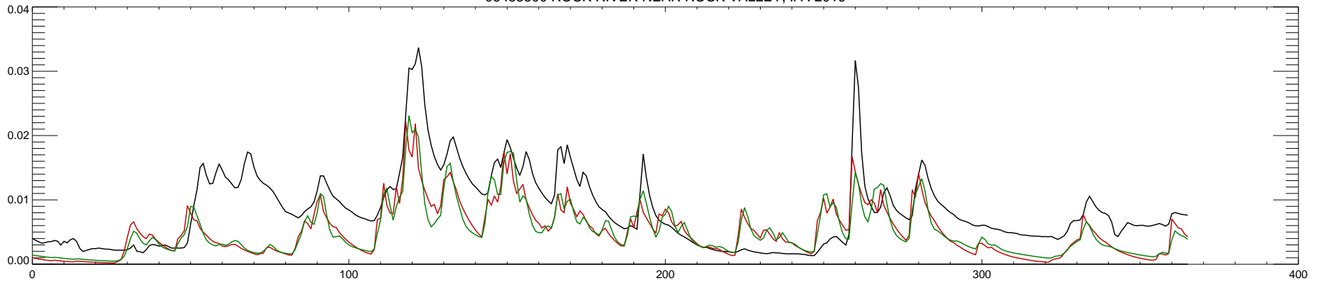
06483500 ROCK RIVER NEAR ROCK VALLEY, IA : 2016
