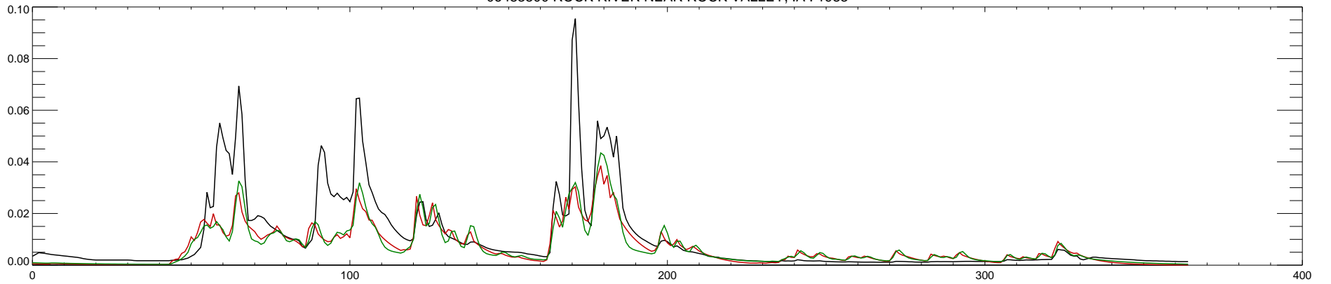
06483500 ROCK RIVER NEAR ROCK VALLEY, IA : 1984
