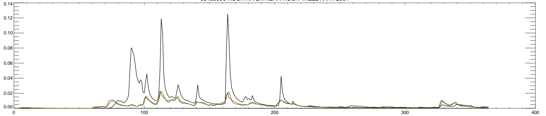
06483500 ROCK RIVER NEAR ROCK VALLEY, IA : 2002
