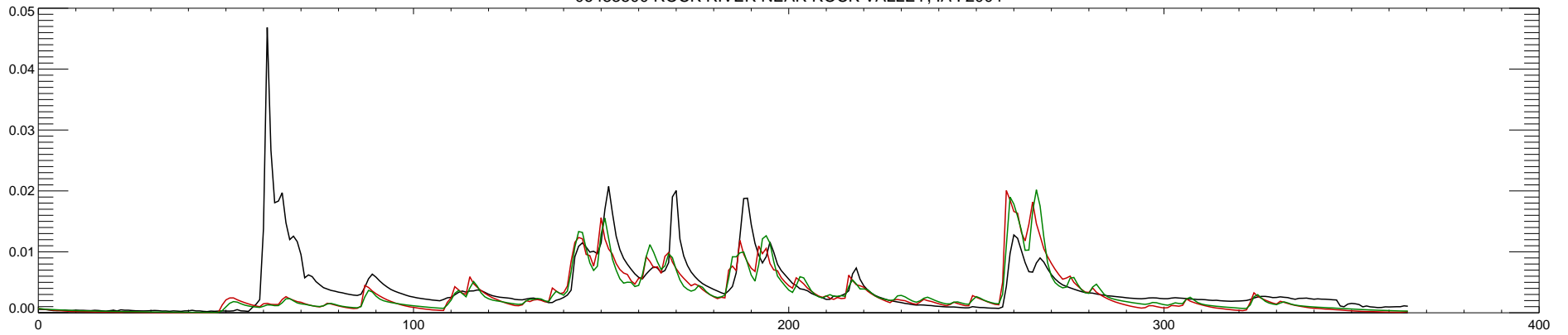
06483500 ROCK RIVER NEAR ROCK VALLEY, IA : 2005
