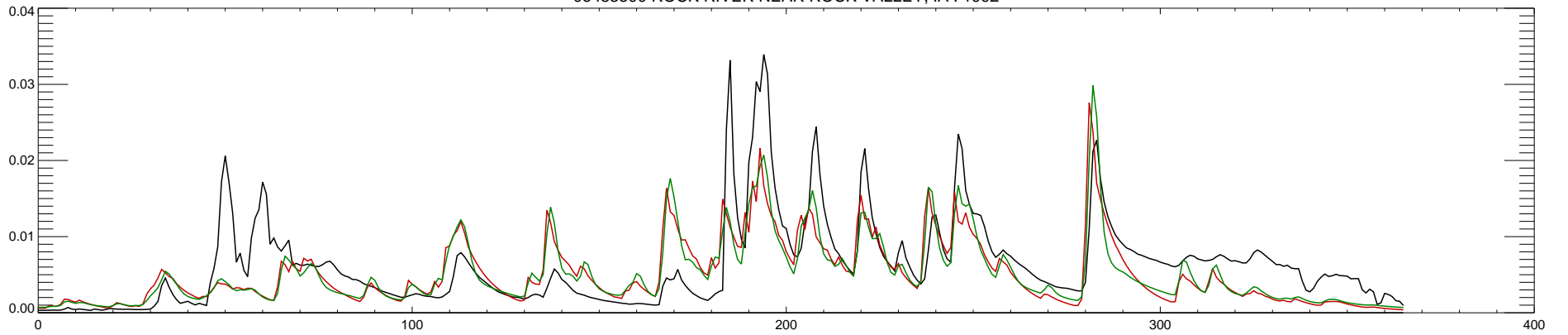
06483500 ROCK RIVER NEAR ROCK VALLEY, IA : 1993
