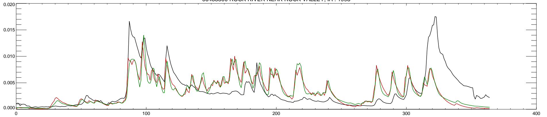
06483500 ROCK RIVER NEAR ROCK VALLEY, IA : 1999
