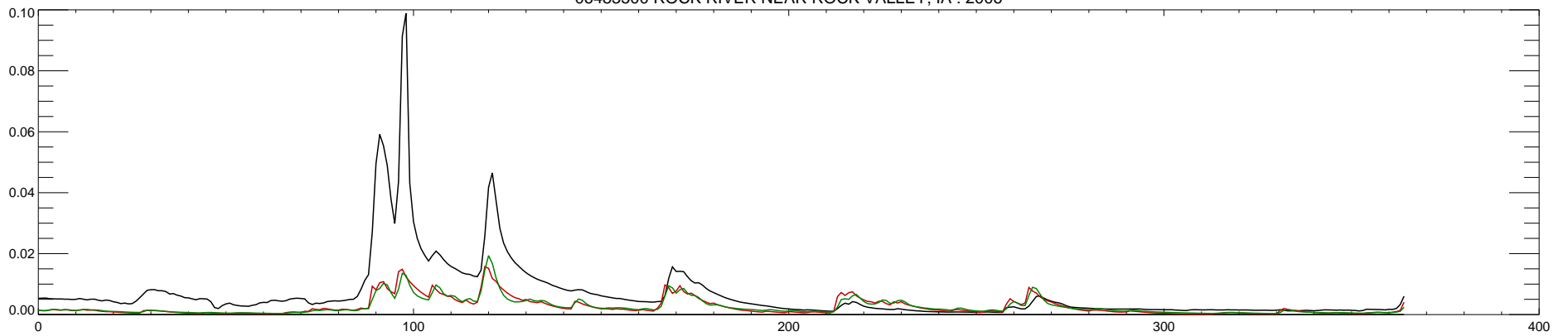
06483500 ROCK RIVER NEAR ROCK VALLEY, IA : 2006
