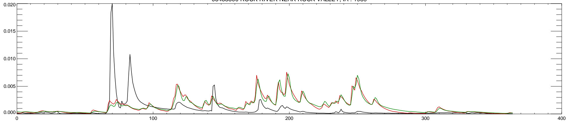
06483500 ROCK RIVER NEAR ROCK VALLEY, IA : 1990
