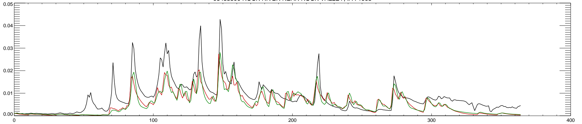
06483500 ROCK RIVER NEAR ROCK VALLEY, IA : 1996
