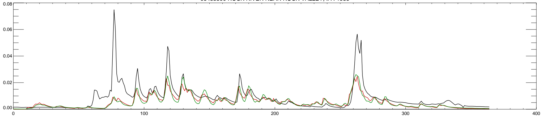
06483500 ROCK RIVER NEAR ROCK VALLEY, IA : 1987
