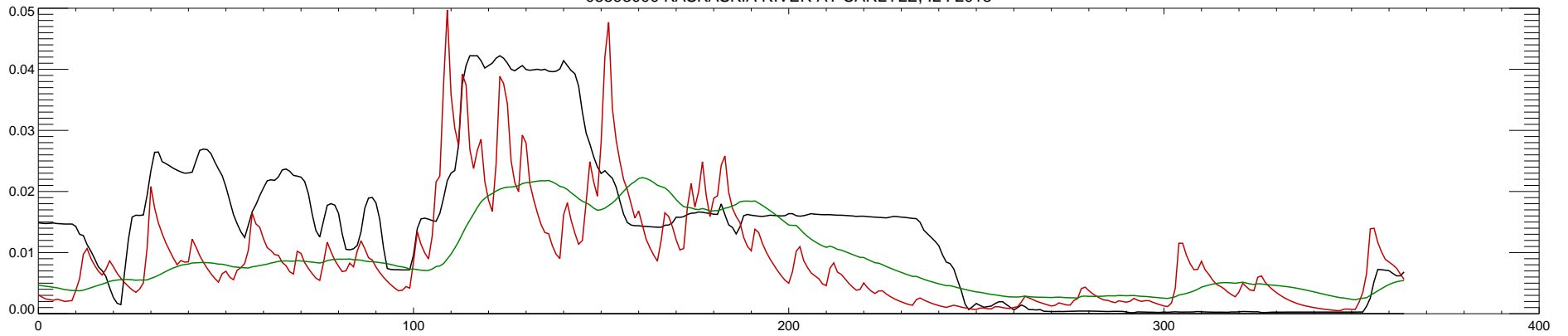
05593000 KASKASKIA RIVER AT CARLYLE, IL : 2014
