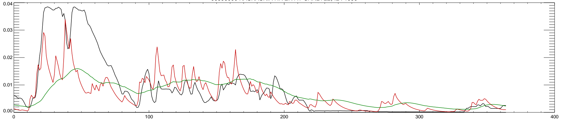
05593000 KASKASKIA RIVER AT CARLYLE, IL : 2000
