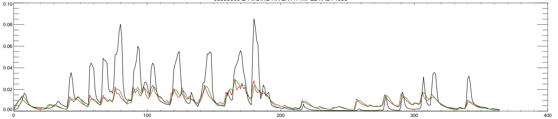
05585000 LA MOINE RIVER AT RIPLEY, IL : 1999
