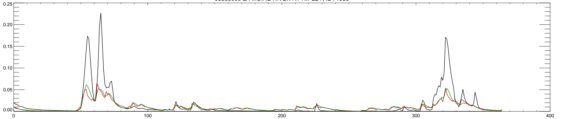
05585000 LA MOINE RIVER AT RIPLEY, IL : 1985
