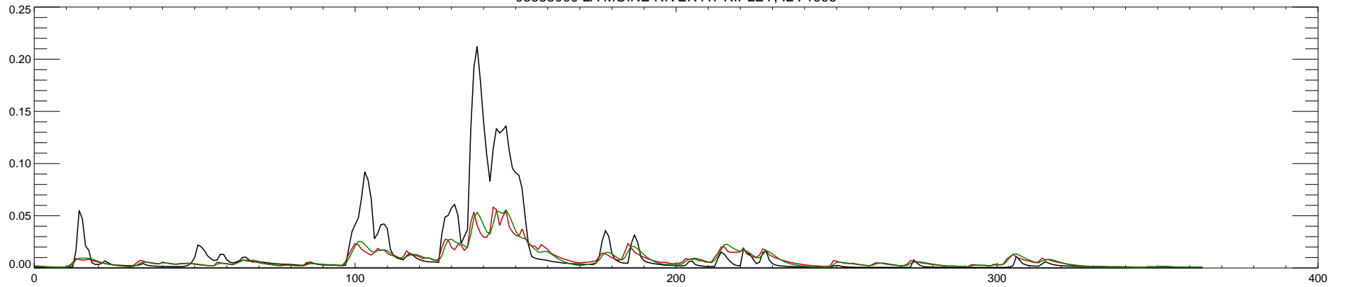
05585000 LA MOINE RIVER AT RIPLEY, IL : 1996
