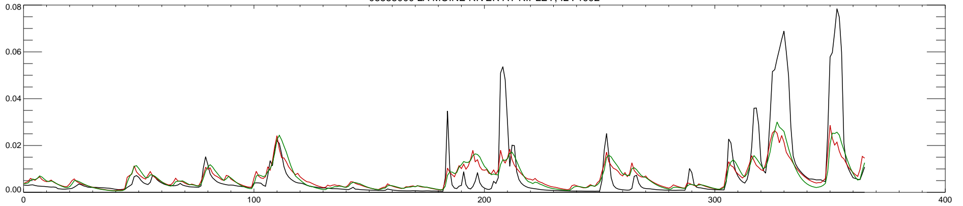
05585000 LA MOINE RIVER AT RIPLEY, IL : 1993
