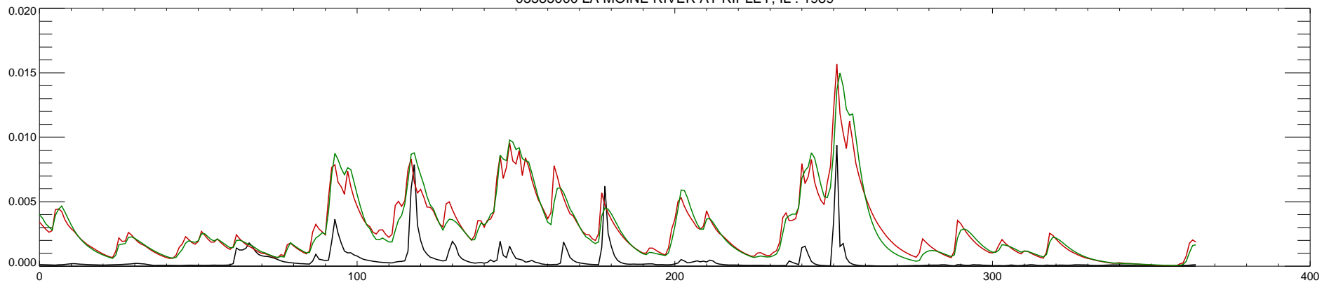
05585000 LA MOINE RIVER AT RIPLEY, IL : 1990
