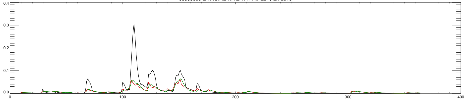
05585000 LA MOINE RIVER AT RIPLEY, IL : 2014
