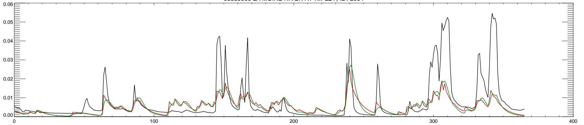
05585000 LA MOINE RIVER AT RIPLEY, IL : 2005
