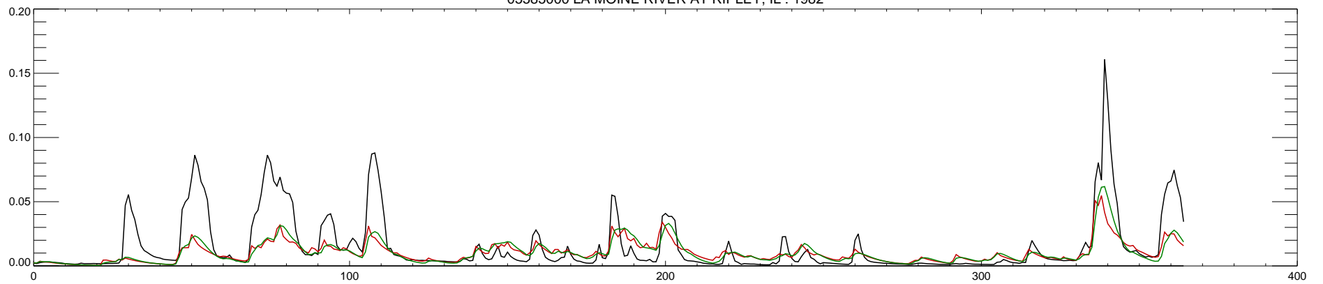
05585000 LA MOINE RIVER AT RIPLEY, IL : 1982
