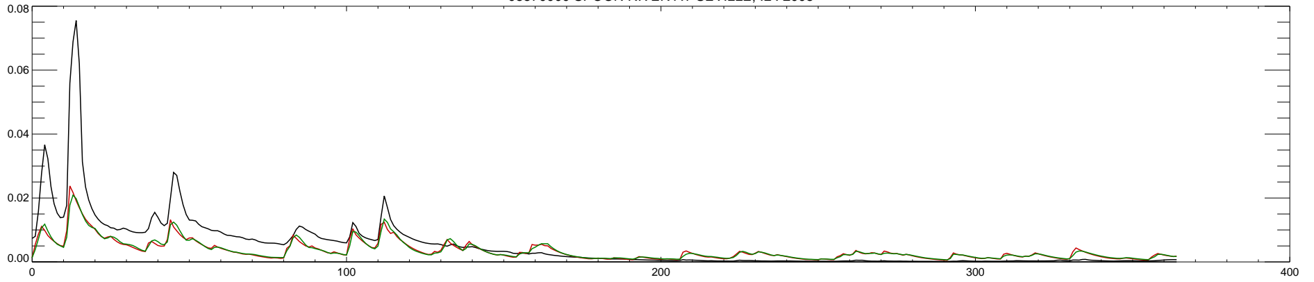
05570000 SPOON RIVER AT SEVILLE, IL : 2006
