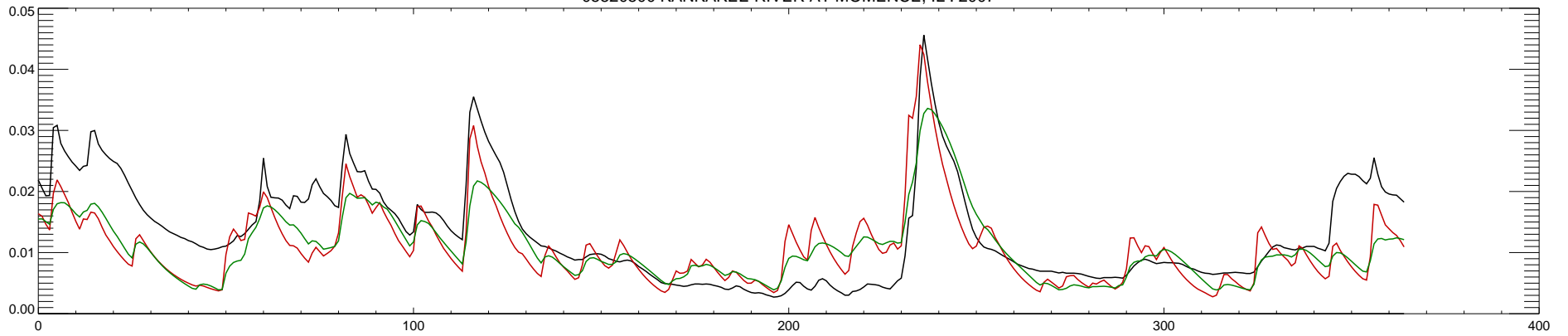
05520500 KANKAKEE RIVER AT MOMENCE, IL : 2008
