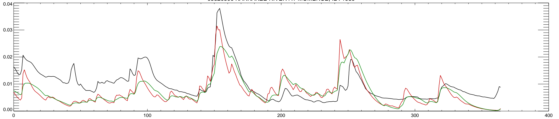
05520500 KANKAKEE RIVER AT MOMENCE, IL : 1990
