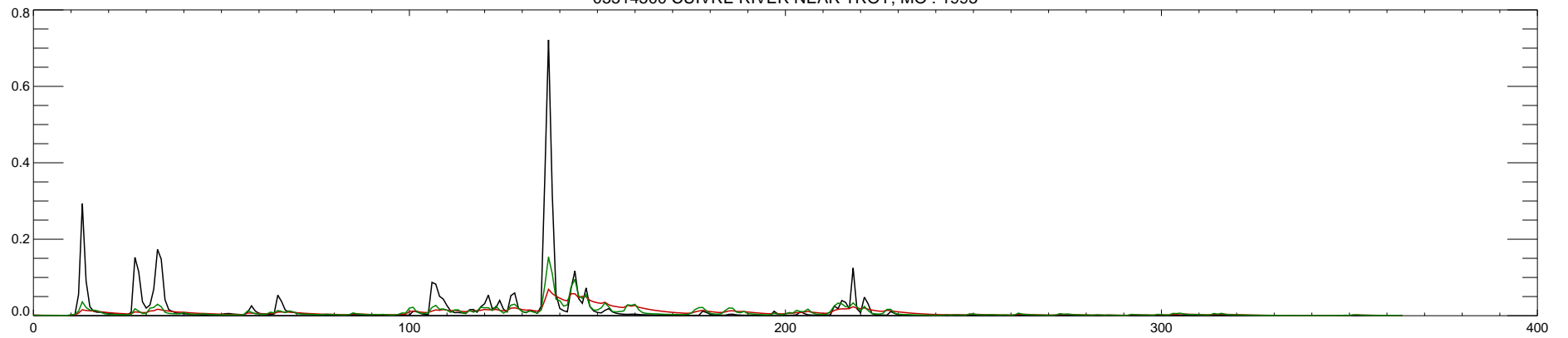
05514500 CUIVRE RIVER NEAR TROY, MO : 1996
