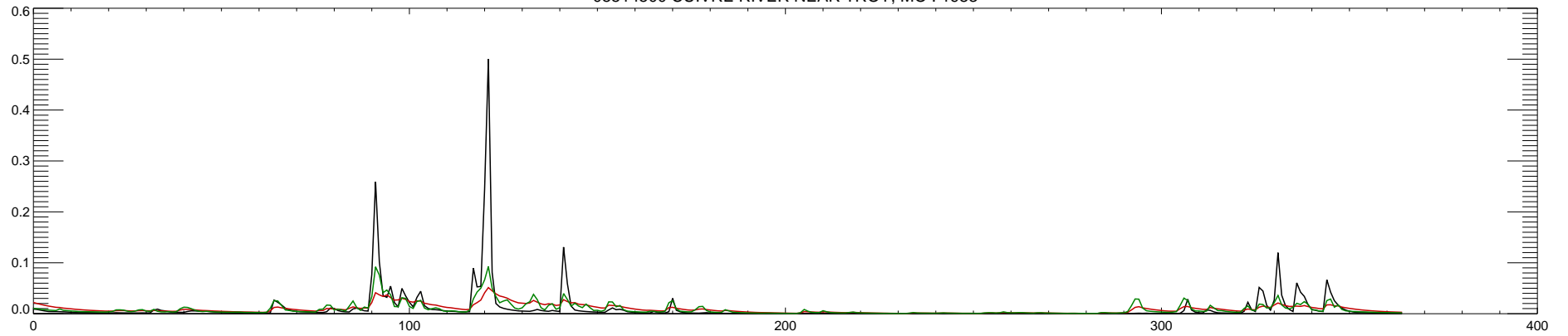
05514500 CUIVRE RIVER NEAR TROY, MO : 1984
