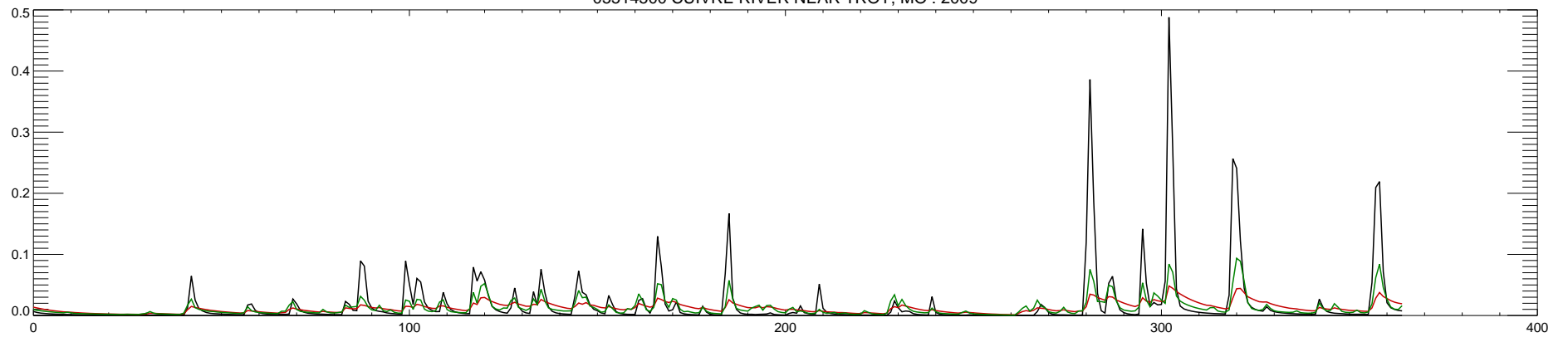
05514500 CUIVRE RIVER NEAR TROY, MO : 2009
