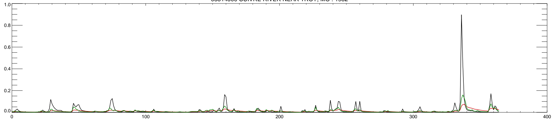
05514500 CUIVRE RIVER NEAR TROY, MO : 1982
