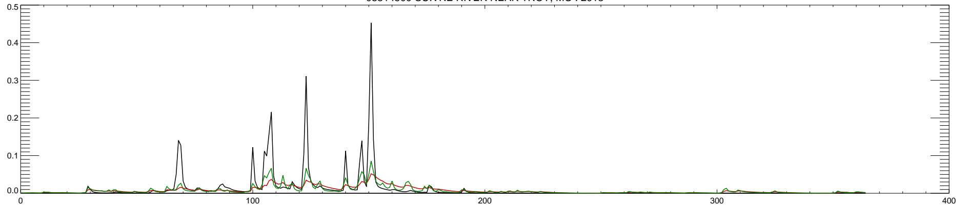
05514500 CUIVRE RIVER NEAR TROY, MO : 2014
