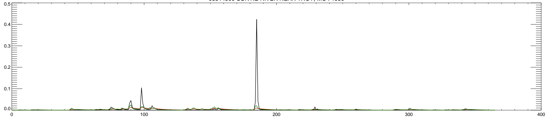
05514500 CUIVRE RIVER NEAR TROY, MO : 1981
