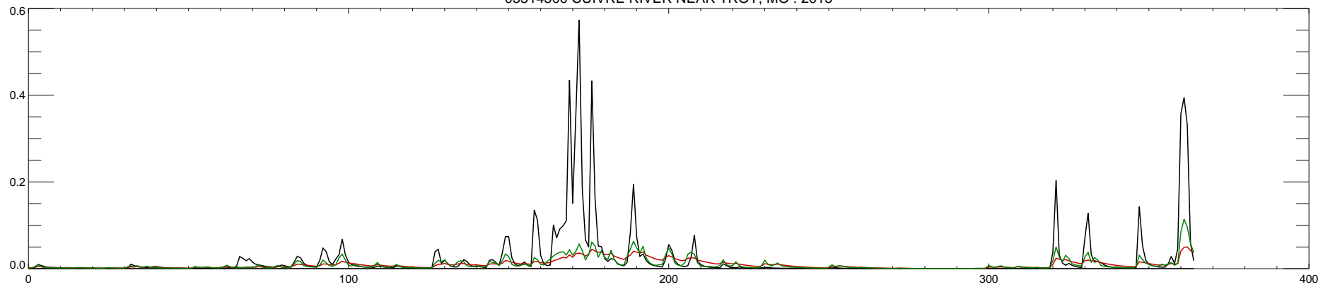
05514500 CUIVRE RIVER NEAR TROY, MO : 2015
