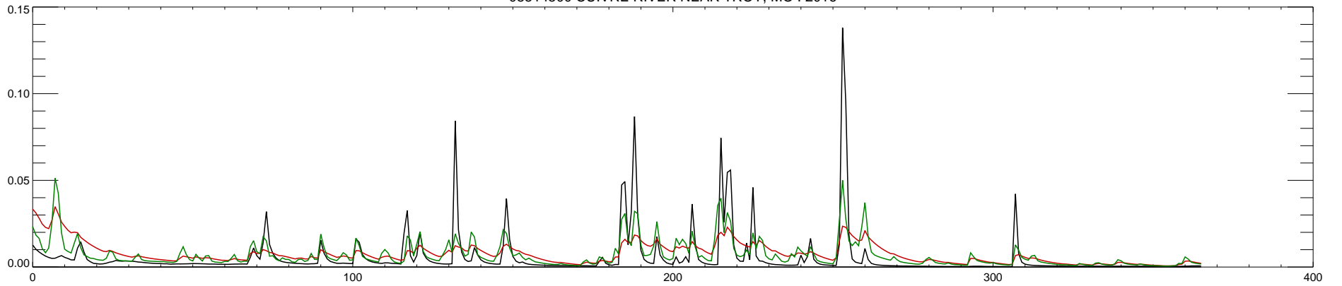
05514500 CUIVRE RIVER NEAR TROY, MO : 2016
