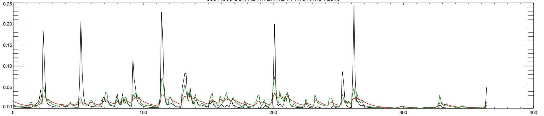
05514500 CUIVRE RIVER NEAR TROY, MO : 2011
