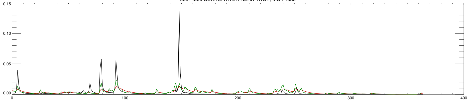
05514500 CUIVRE RIVER NEAR TROY, MO : 1990
