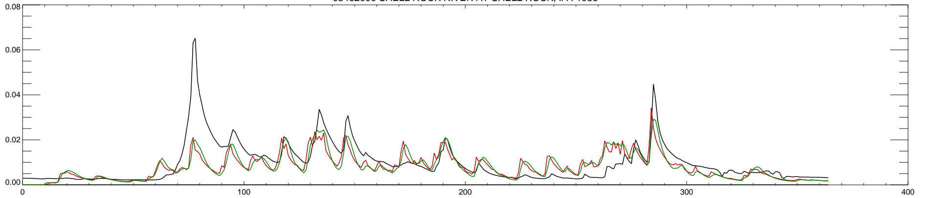
05462000 SHELL ROCK RIVER AT SHELL ROCK, IA : 1987
