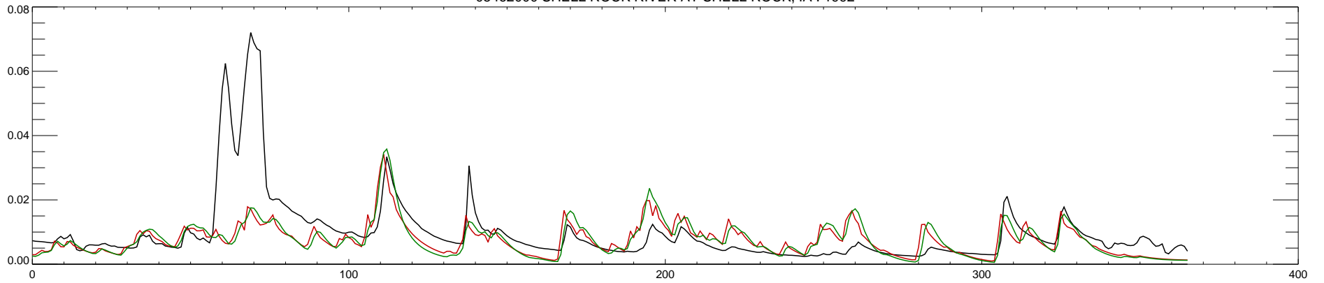
05462000 SHELL ROCK RIVER AT SHELL ROCK, IA : 1993
