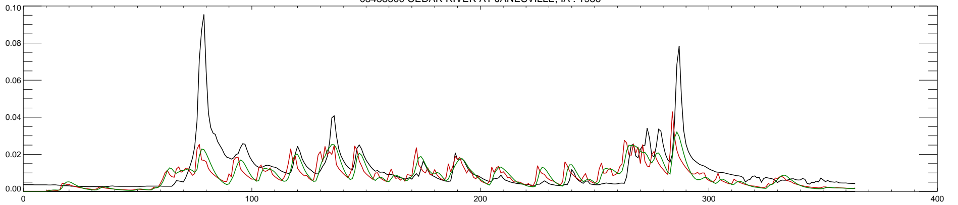
05458500 CEDAR RIVER AT JANESVILLE, IA : 1987
