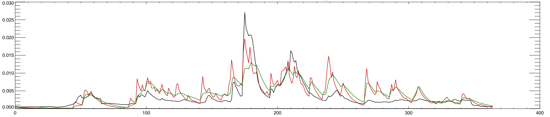
05451500 IOWA RIVER AT MARSHALLTOWN, IA : 1982
