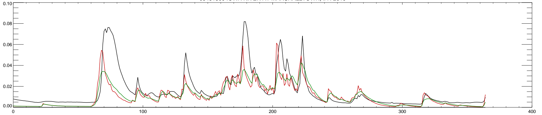
05451500 IOWA RIVER AT MARSHALLTOWN, IA : 2011
