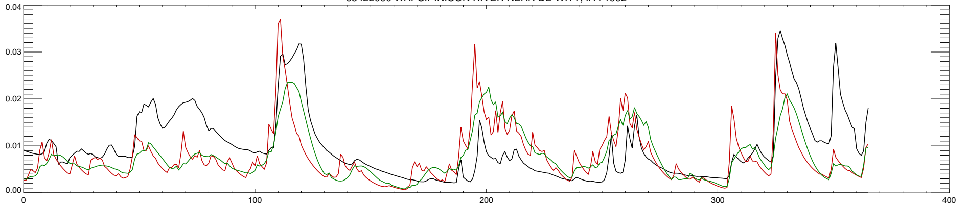
05422000 WAPSIPINICON RIVER NEAR DE WITT, IA : 1993
