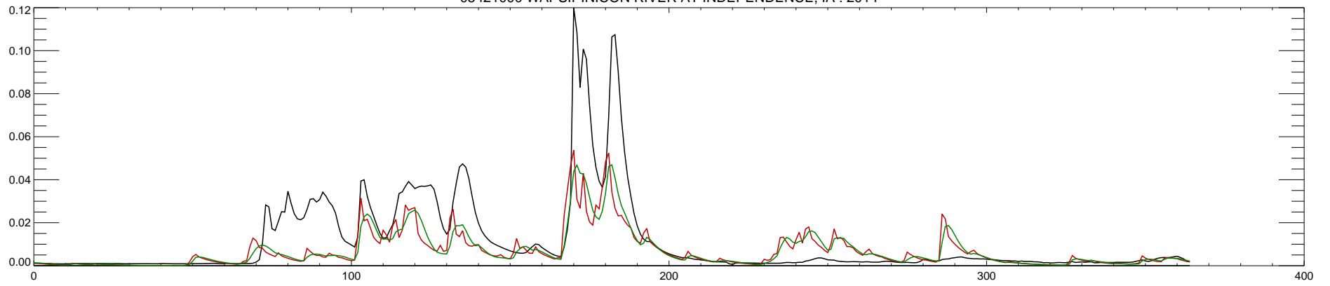
05421000 WAPSIPINICON RIVER AT INDEPENDENCE, IA : 2015
