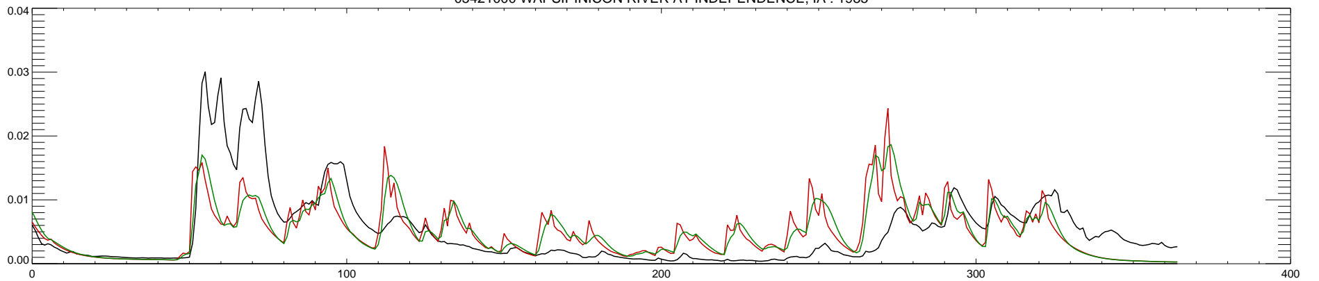
05421000 WAPSIPINICON RIVER AT INDEPENDENCE, IA : 1985
