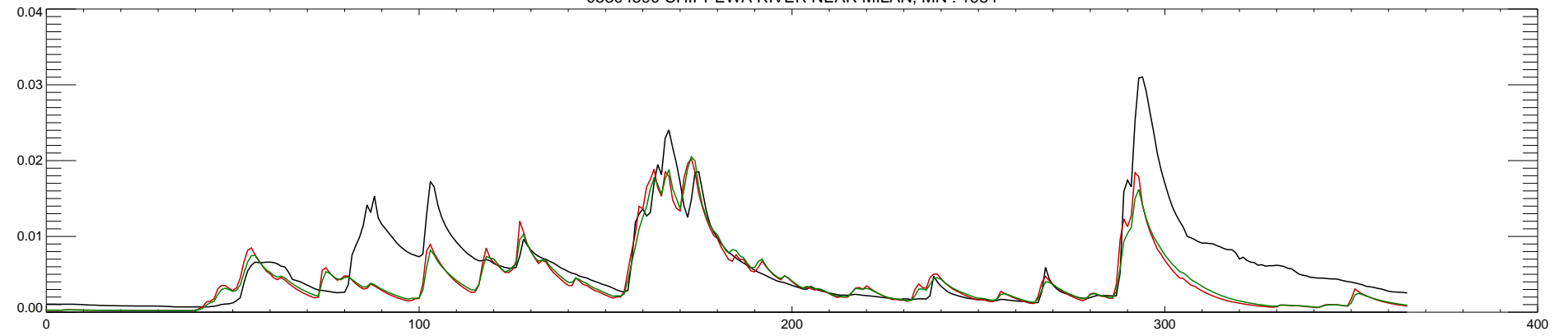
05304500 CHIPPEWA RIVER NEAR MILAN, MN : 1985
