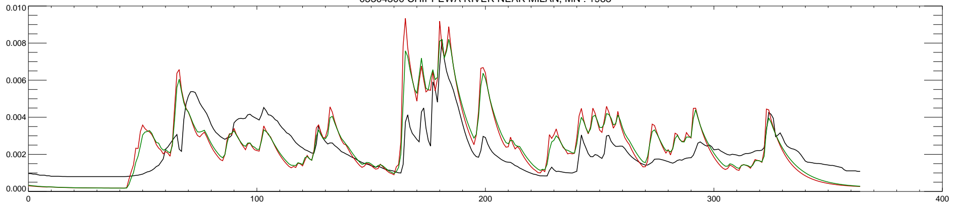
05304500 CHIPPEWA RIVER NEAR MILAN, MN : 1984
