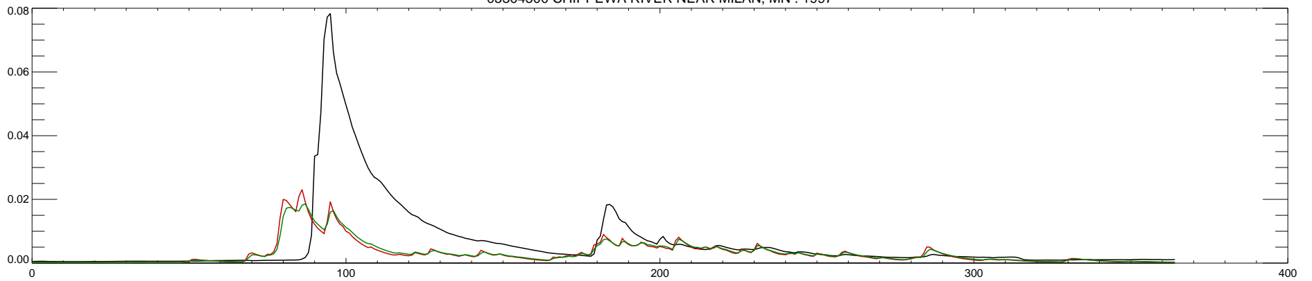
05304500 CHIPPEWA RIVER NEAR MILAN, MN : 1997
