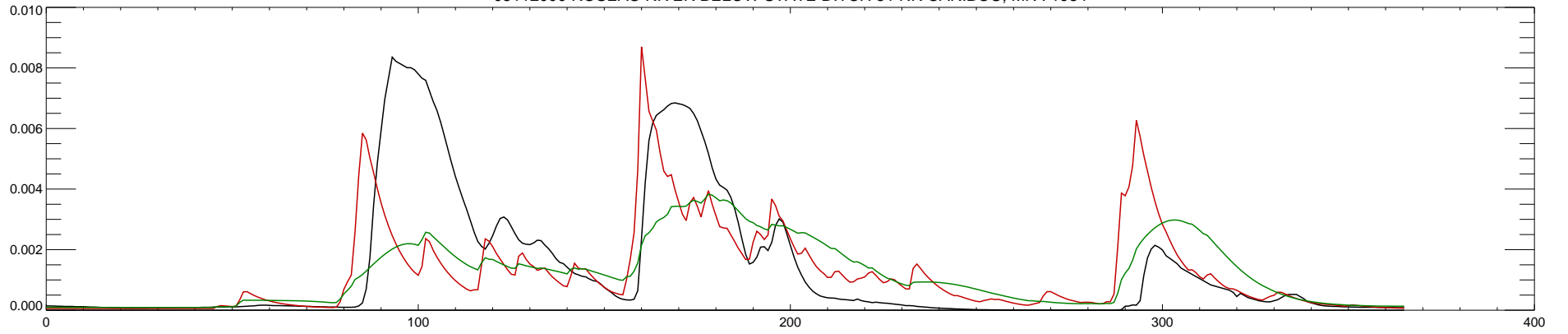
05112000 ROSEAU RIVER BELOW STATE DITCH 51 NR CARIBOU, MN : 1985
