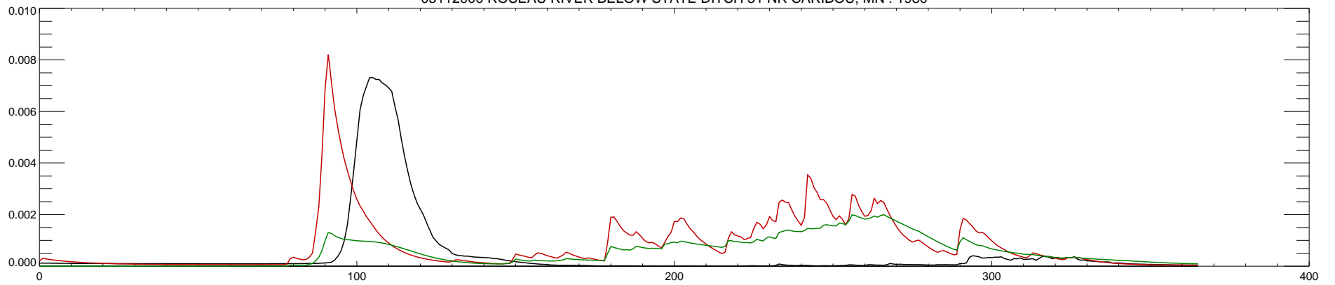
05112000 ROSEAU RIVER BELOW STATE DITCH 51 NR CARIBOU, MN : 1981
