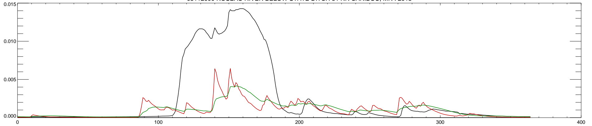
05112000 ROSEAU RIVER BELOW STATE DITCH 51 NR CARIBOU, MN : 2014
