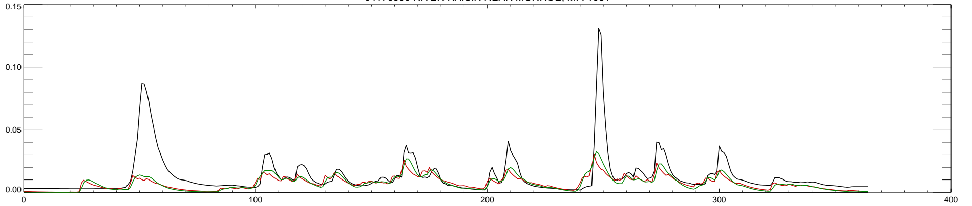
04176500 RIVER RAISIN NEAR MONROE, MI : 1982
