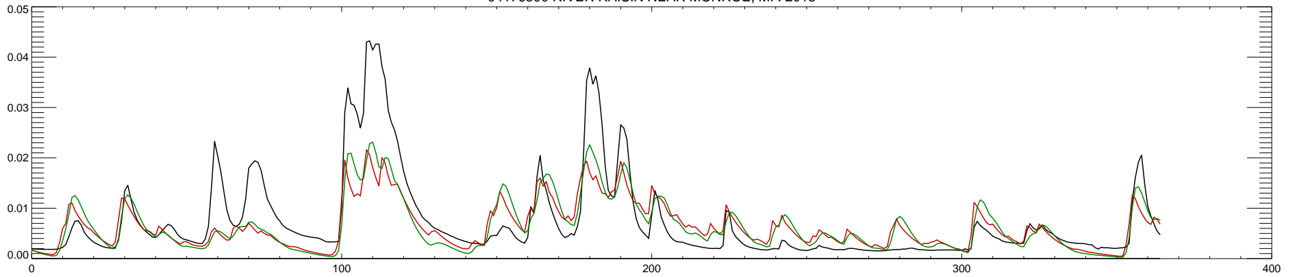
04176500 RIVER RAISIN NEAR MONROE, MI : 2014
