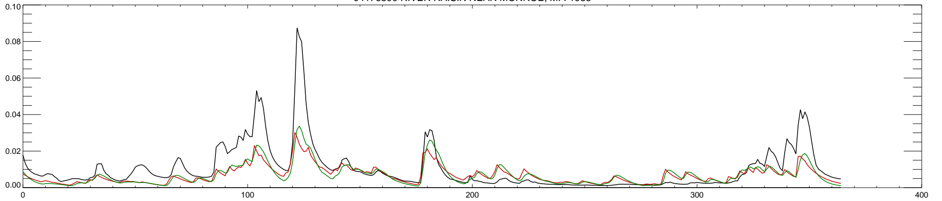
04176500 RIVER RAISIN NEAR MONROE, MI : 1984
