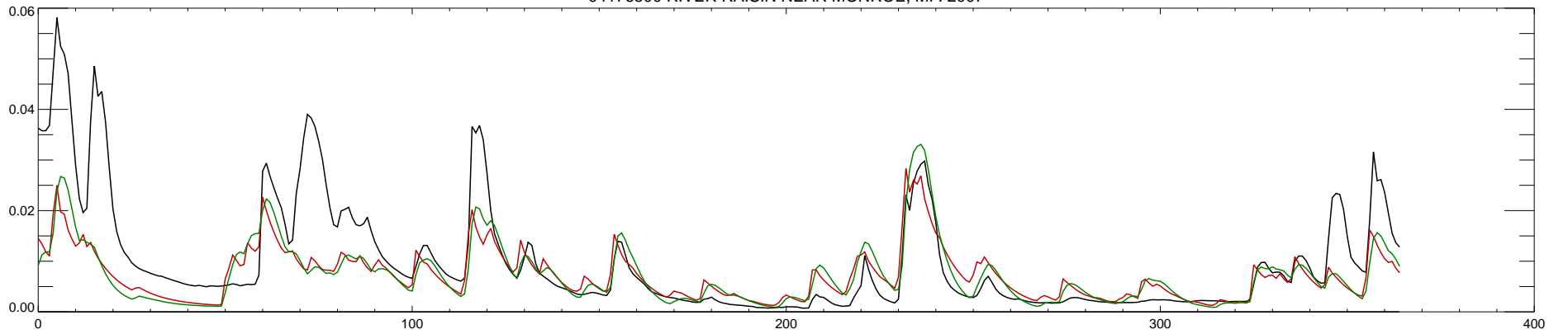
04176500 RIVER RAISIN NEAR MONROE, MI : 2008
