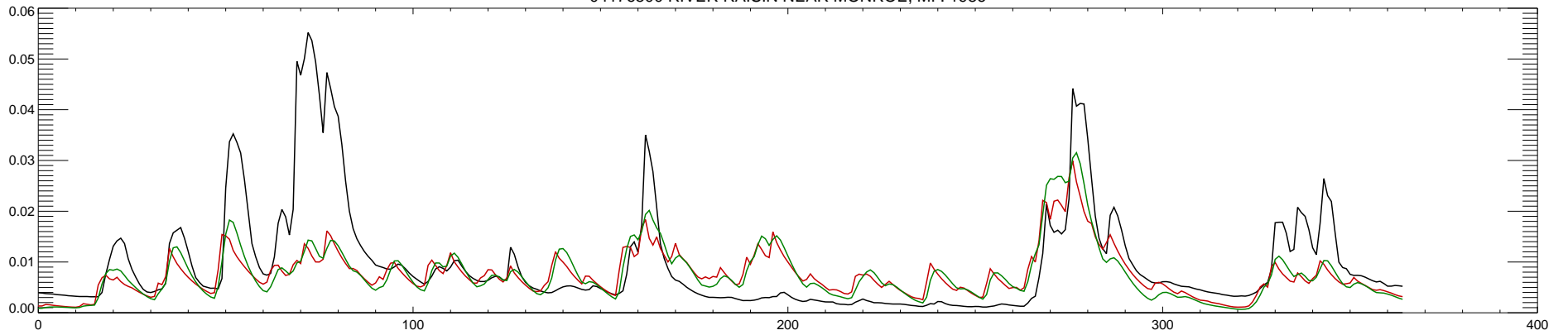
04176500 RIVER RAISIN NEAR MONROE, MI : 1987
