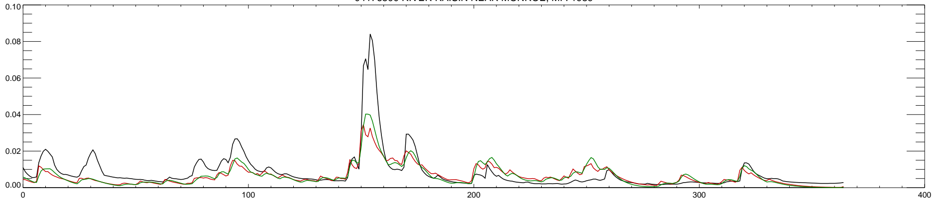
04176500 RIVER RAISIN NEAR MONROE, MI : 1990
