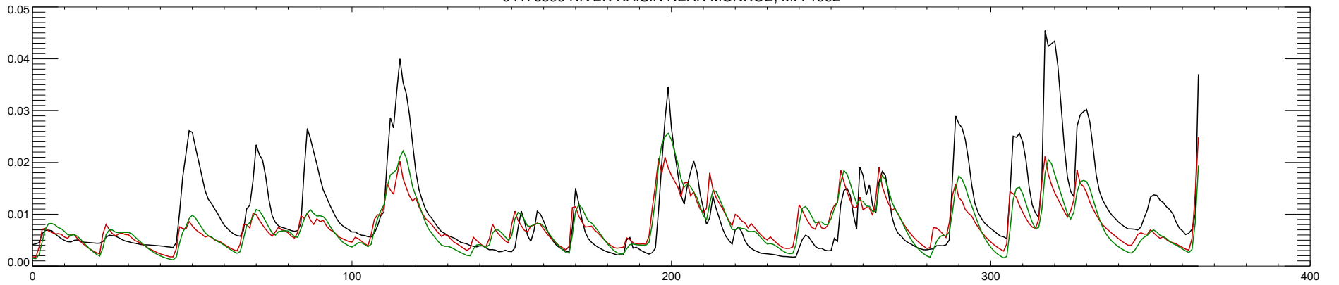
04176500 RIVER RAISIN NEAR MONROE, MI : 1993
