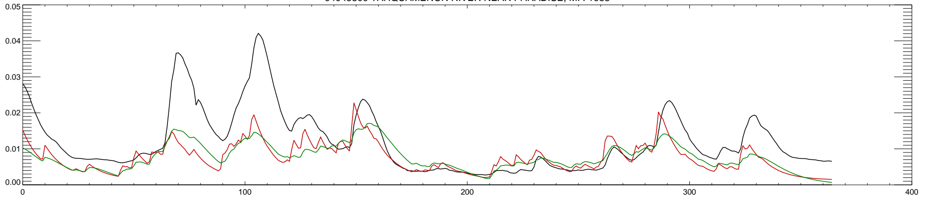
04045500 TAHQUAMENON RIVER NEAR PARADISE, MI : 1984
