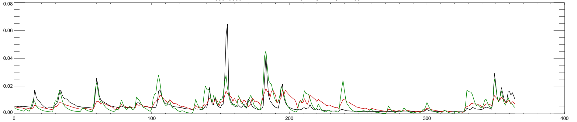
03349000 WHITE RIVER AT NOBLESVILLE, IN : 1988
