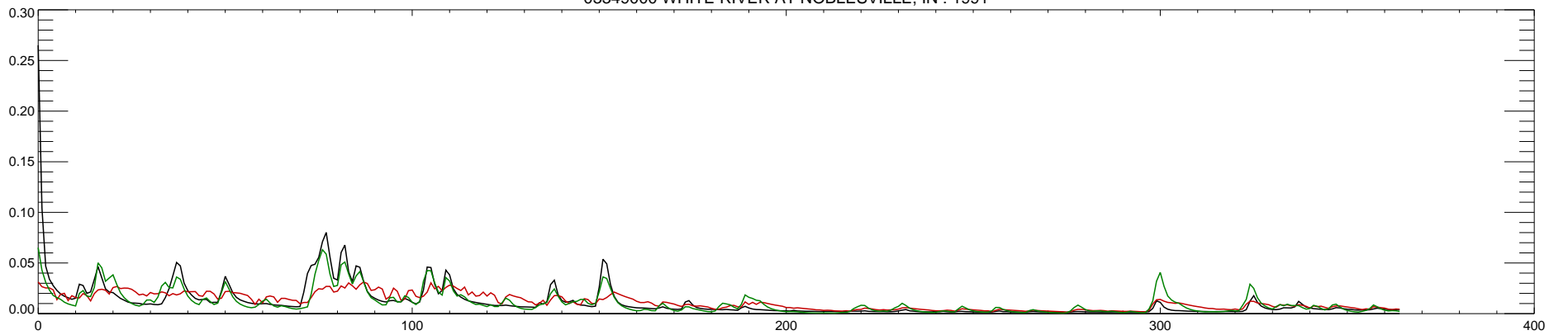
03349000 WHITE RIVER AT NOBLESVILLE, IN : 1991
