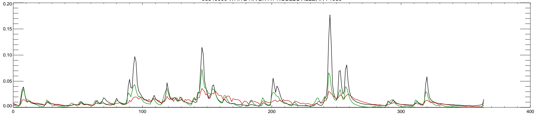
03349000 WHITE RIVER AT NOBLESVILLE, IN : 1990
