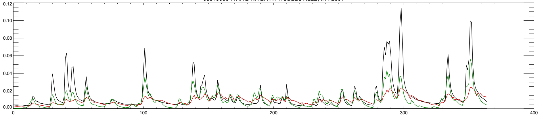
03349000 WHITE RIVER AT NOBLESVILLE, IN : 2002
