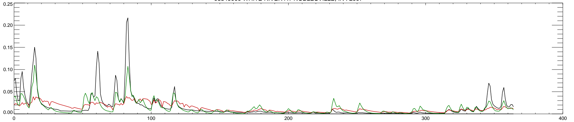
03349000 WHITE RIVER AT NOBLESVILLE, IN : 2008
