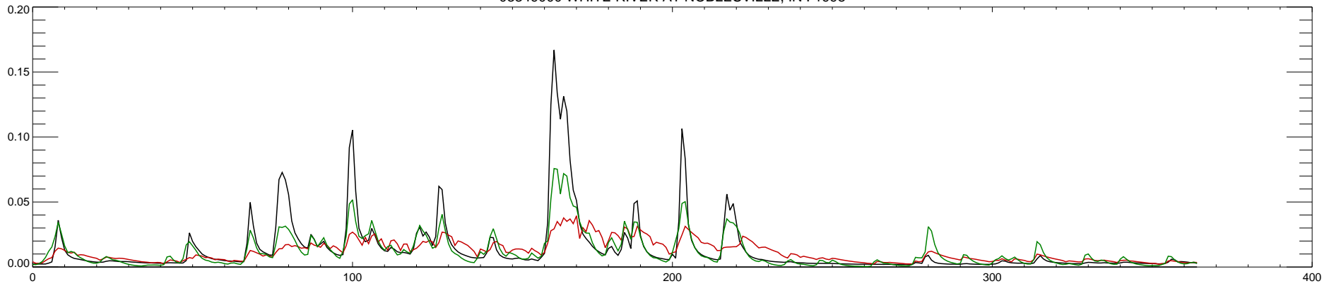
03349000 WHITE RIVER AT NOBLESVILLE, IN : 1999
