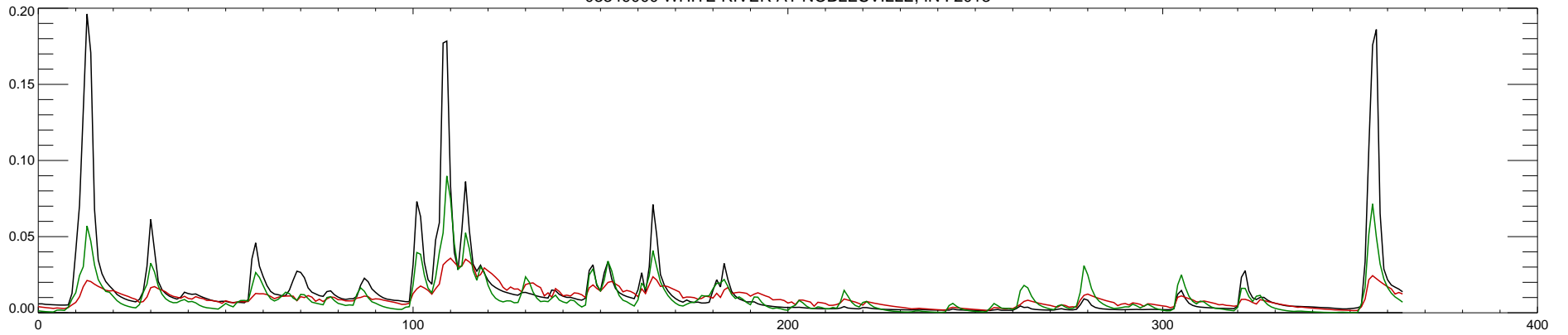
03349000 WHITE RIVER AT NOBLESVILLE, IN : 2014
