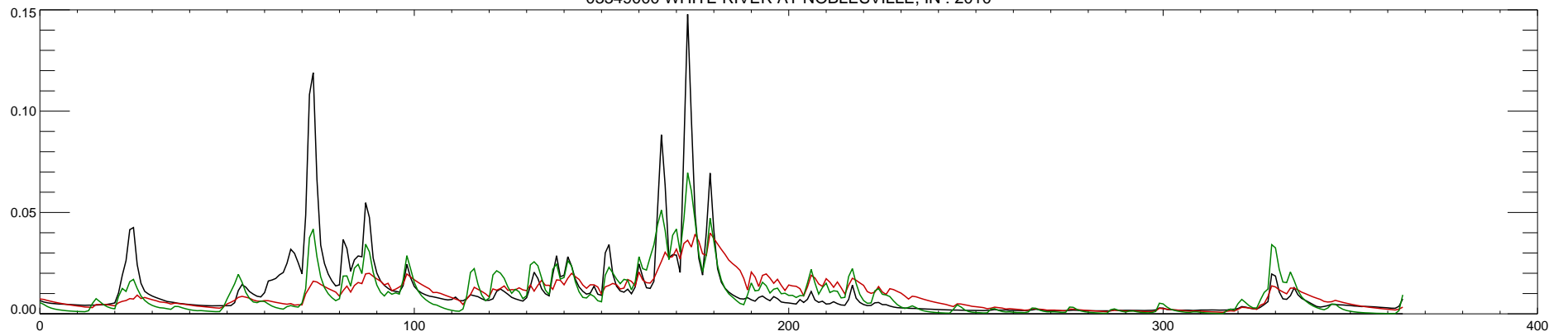
03349000 WHITE RIVER AT NOBLESVILLE, IN : 2011
