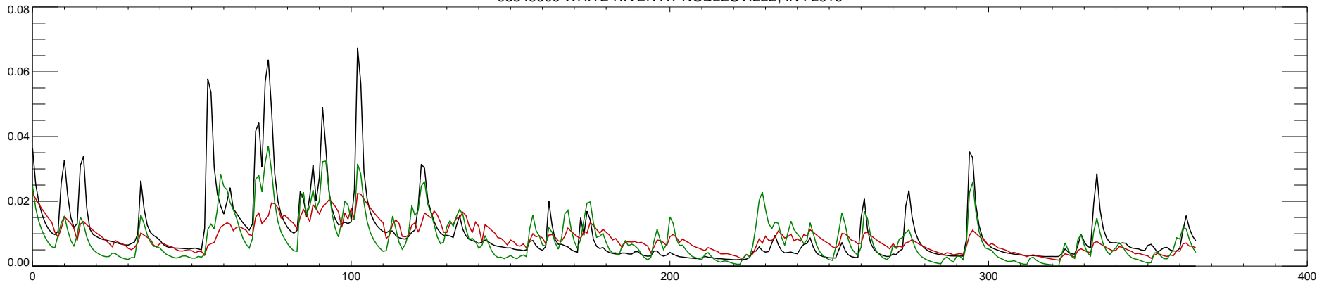
03349000 WHITE RIVER AT NOBLESVILLE, IN : 2016
