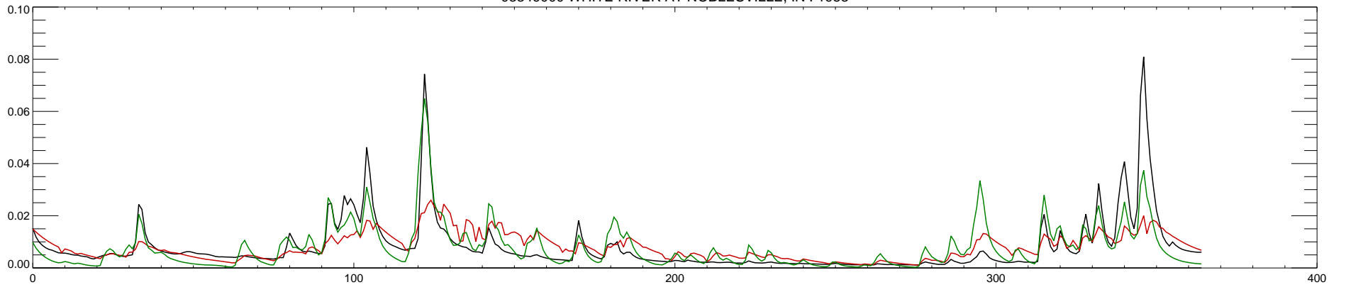
03349000 WHITE RIVER AT NOBLESVILLE, IN : 1984
