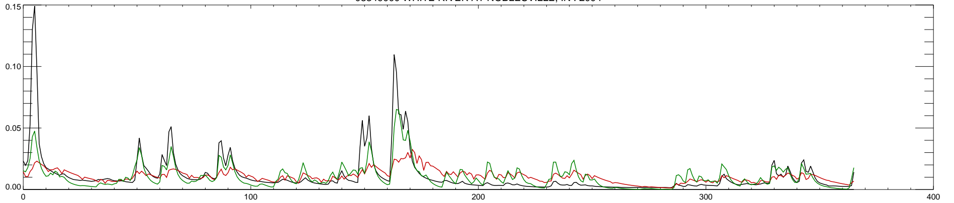
03349000 WHITE RIVER AT NOBLESVILLE, IN : 2005
