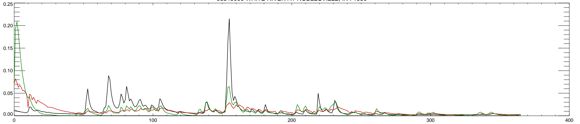
03349000 WHITE RIVER AT NOBLESVILLE, IN : 1981
