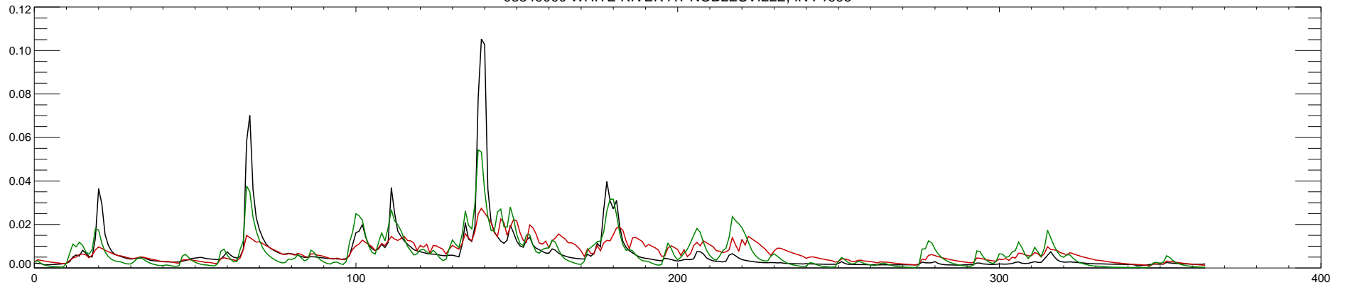
03349000 WHITE RIVER AT NOBLESVILLE, IN : 1996
