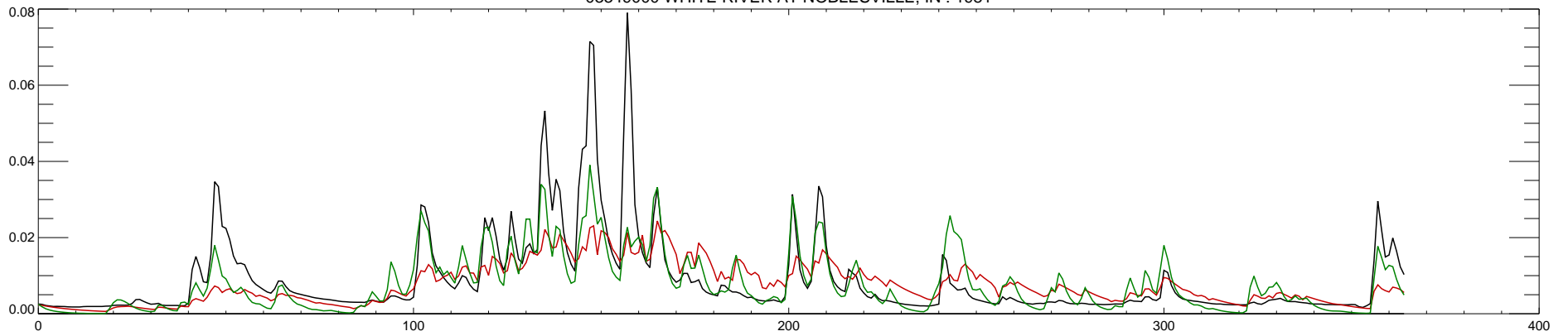
03349000 WHITE RIVER AT NOBLESVILLE, IN : 1982
