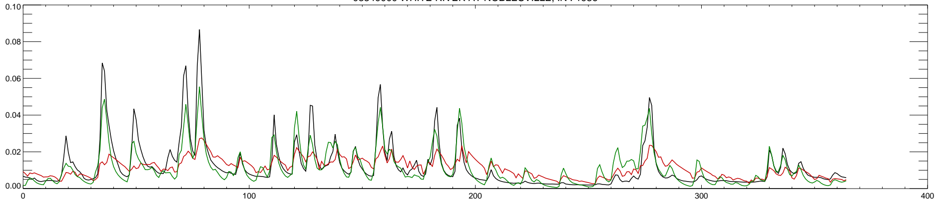
03349000 WHITE RIVER AT NOBLESVILLE, IN : 1987
