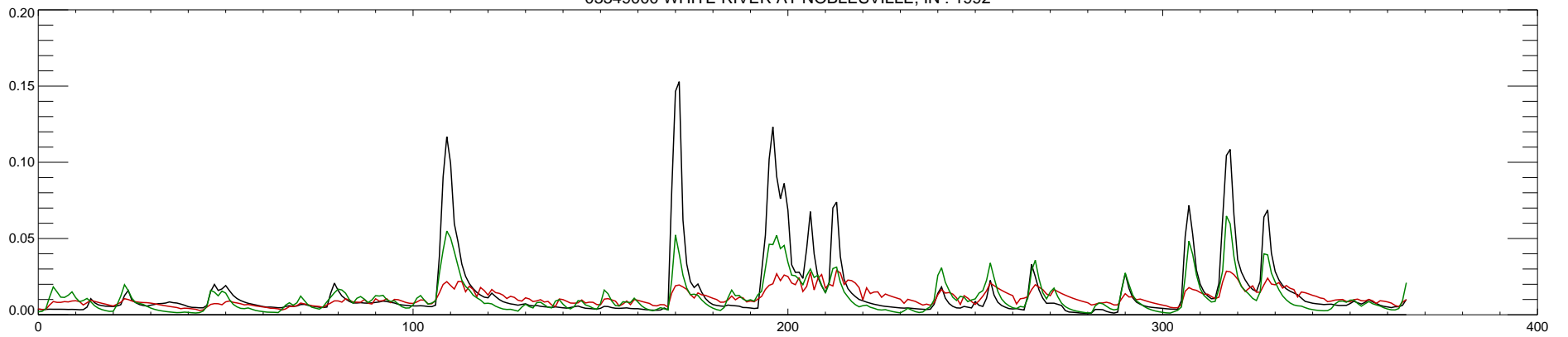
03349000 WHITE RIVER AT NOBLESVILLE, IN : 1993
