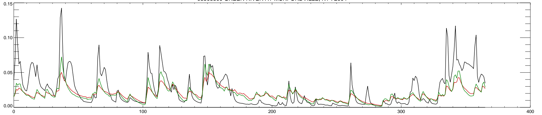
03308500 GREEN RIVER AT MUNFORDVILLE, KY : 2005
