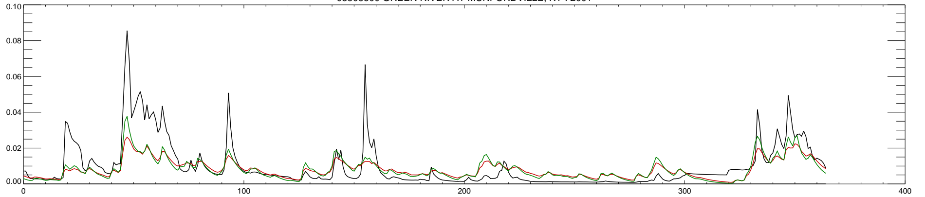
03308500 GREEN RIVER AT MUNFORDVILLE, KY : 2002
