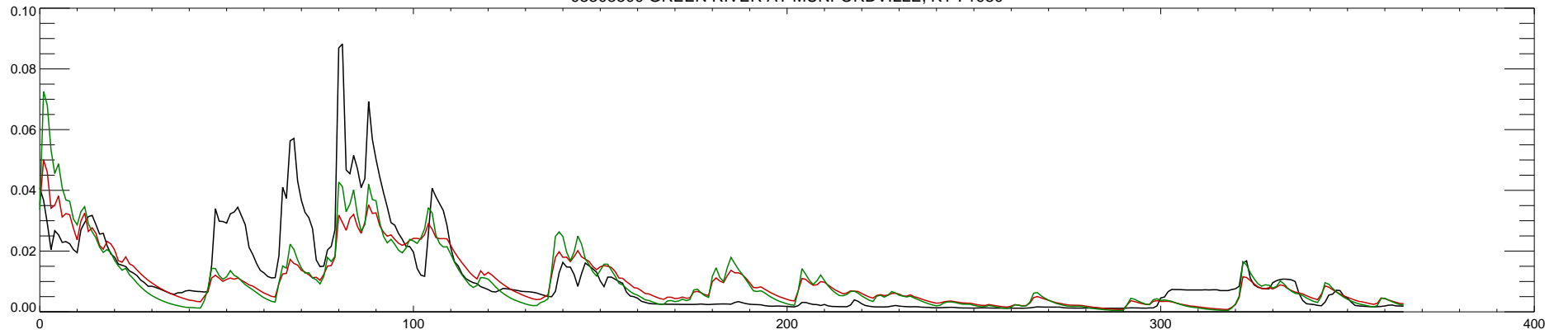
03308500 GREEN RIVER AT MUNFORDVILLE, KY : 1981
