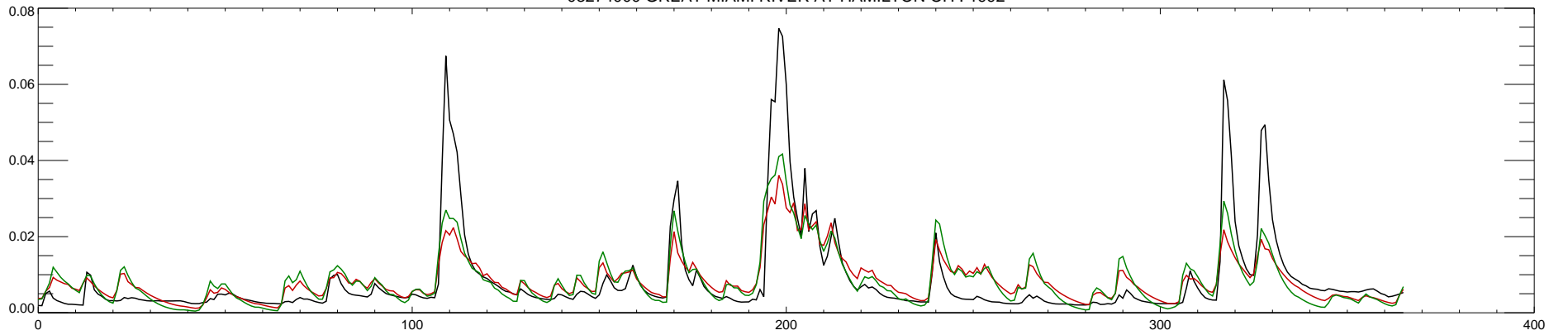
03274000 GREAT MIAMI RIVER AT HAMILTON OH : 1993
