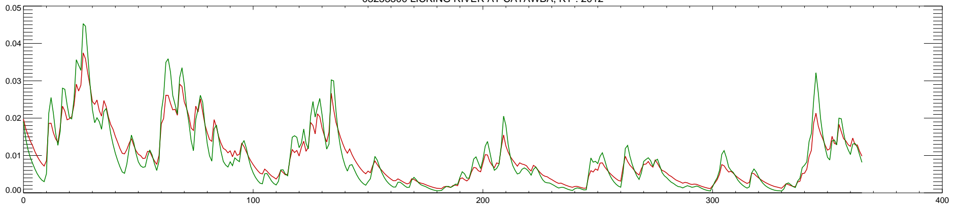
03253500 LICKING RIVER AT CATAWBA, KY : 2012
