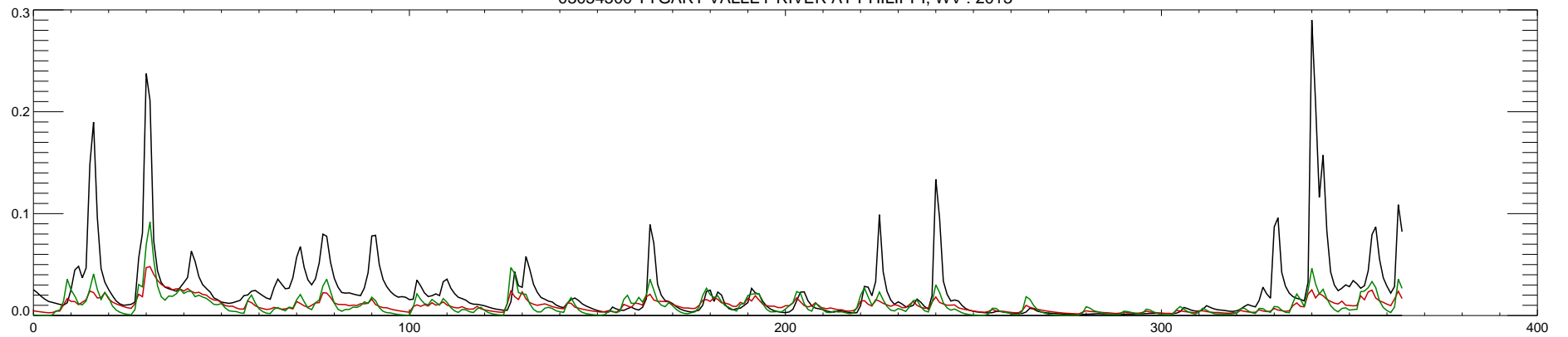
03054500 TYGART VALLEY RIVER AT PHILIPPI, WV : 2014
