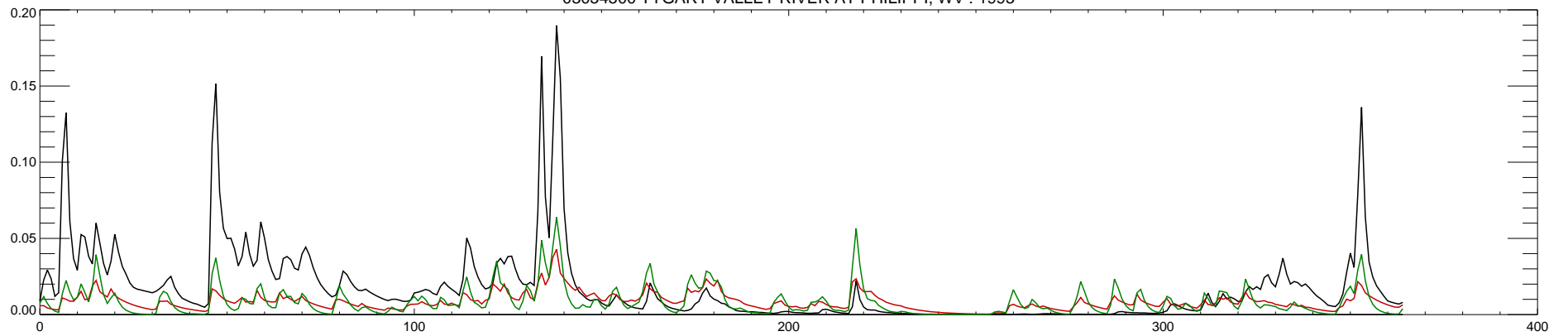
03054500 TYGART VALLEY RIVER AT PHILIPPI, WV : 1996
