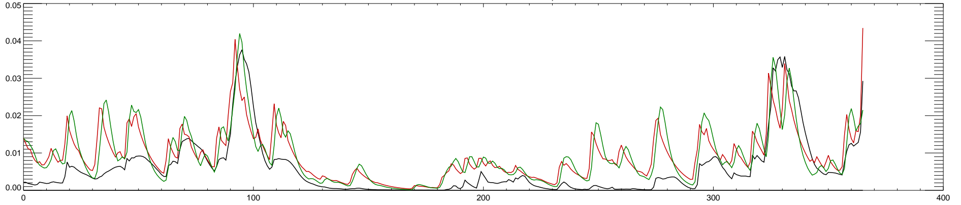
02482000 PEARL RIVER AT EDINBURG, MS : 1988
