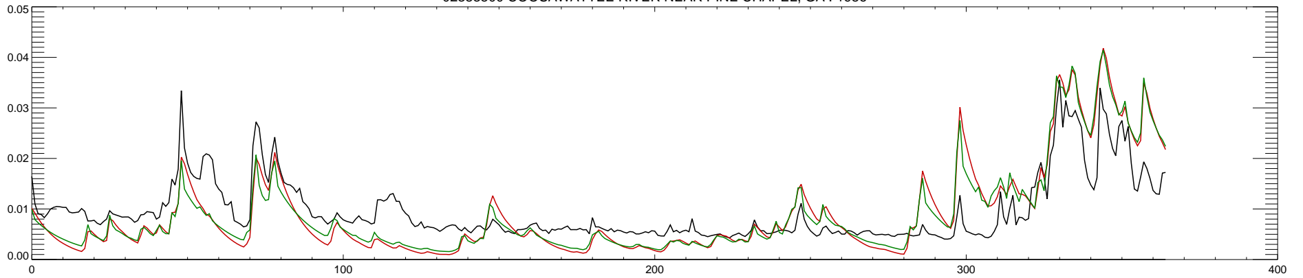
02383500 COOSAWATTEE RIVER NEAR PINE CHAPEL, GA : 1987
