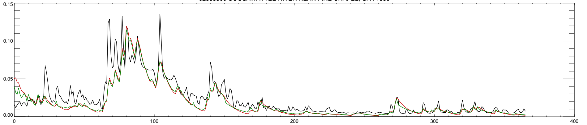
02383500 COOSAWATTEE RIVER NEAR PINE CHAPEL, GA : 1981
