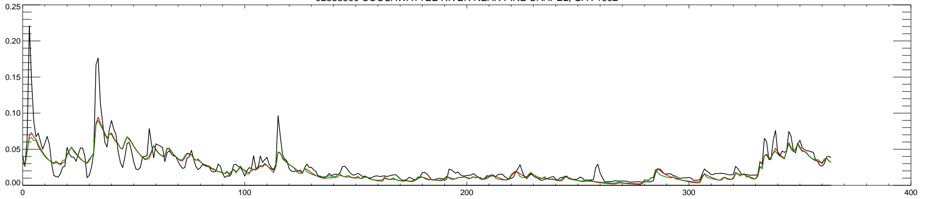
02383500 COOSAWATTEE RIVER NEAR PINE CHAPEL, GA : 1982
