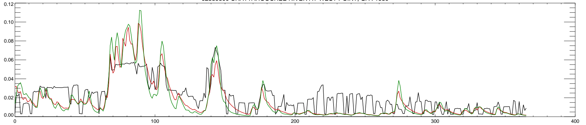
02339500 CHATTAHOOCHEE RIVER AT WEST POINT, GA : 1981
