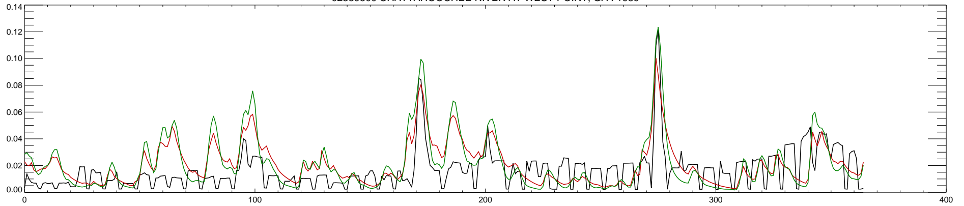
02339500 CHATTAHOOCHEE RIVER AT WEST POINT, GA : 1990
