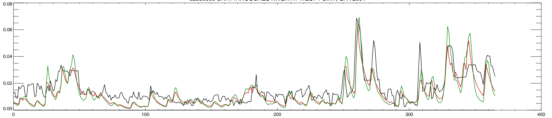
02339500 CHATTAHOOCHEE RIVER AT WEST POINT, GA : 2005
