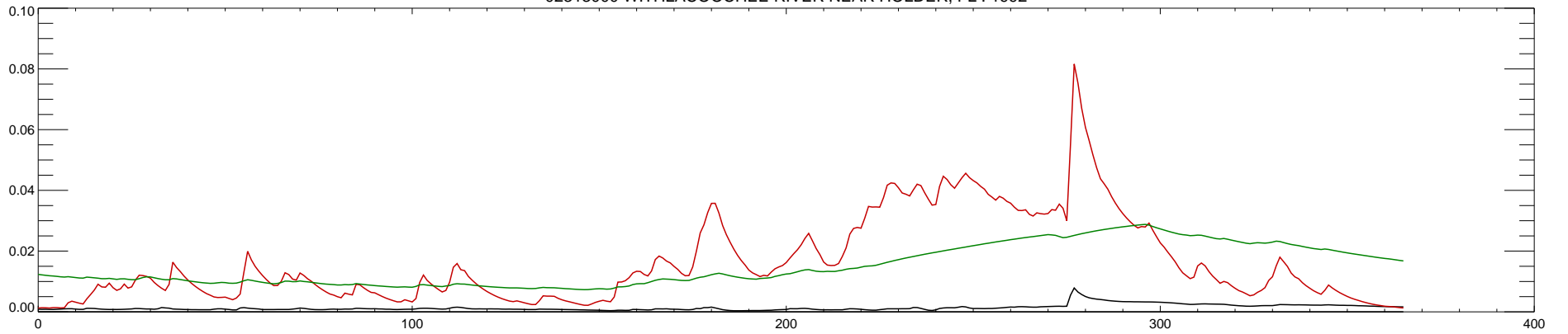
02313000 WITHLACOOCHEE RIVER NEAR HOLDER, FL : 1993
