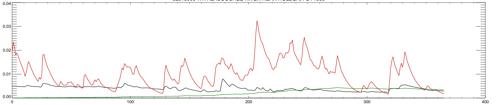
02313000 WITHLACOOCHEE RIVER NEAR HOLDER, FL : 1981
