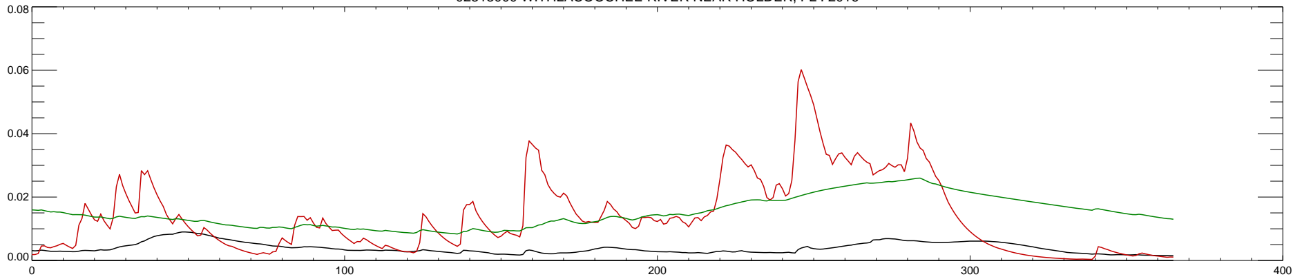
02313000 WITHLACOOCHEE RIVER NEAR HOLDER, FL : 2016
