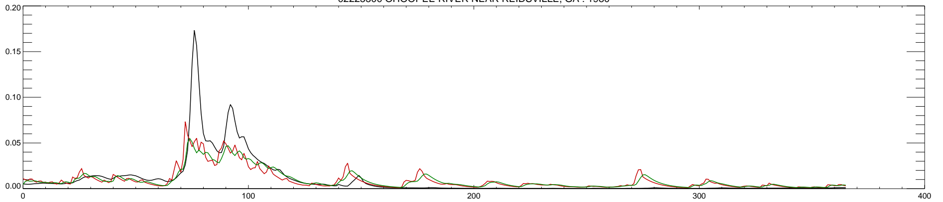
02225500 OHOOPEE RIVER NEAR REIDSVILLE, GA : 1981
