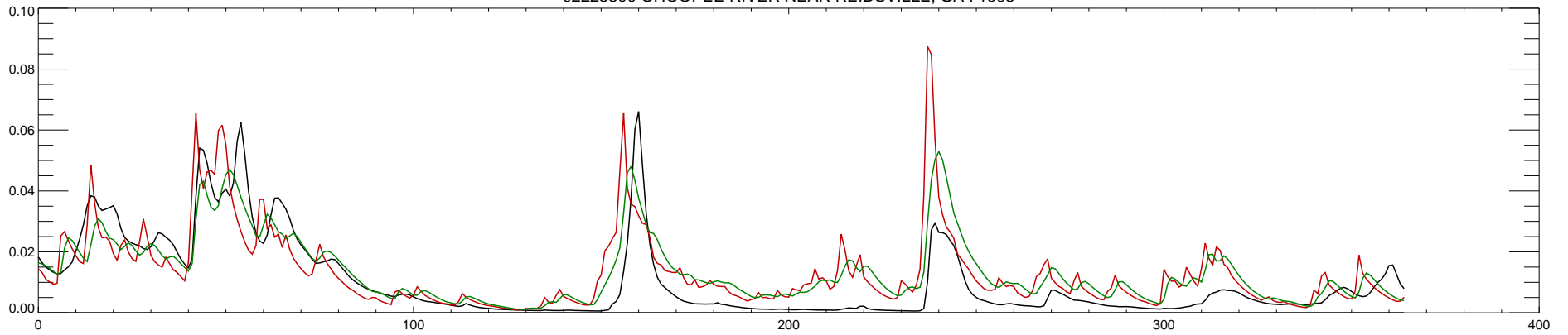
02225500 OHOOPEE RIVER NEAR REIDSVILLE, GA : 1996
