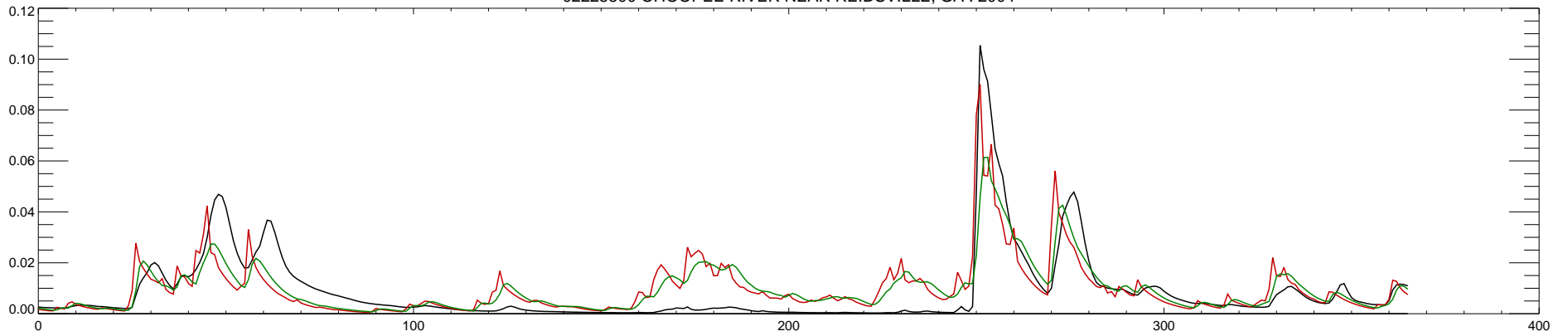
02225500 OHOOPEE RIVER NEAR REIDSVILLE, GA : 2005
