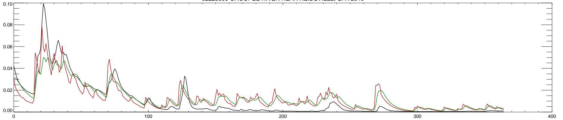
02225500 OHOOPEE RIVER NEAR REIDSVILLE, GA : 2011
