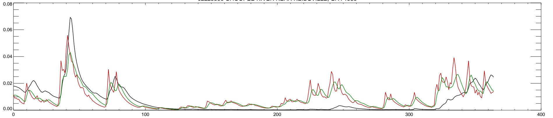
02225500 OHOOPEE RIVER NEAR REIDSVILLE, GA : 1987
