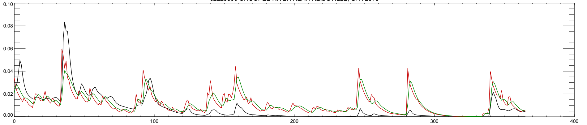
02225500 OHOOPEE RIVER NEAR REIDSVILLE, GA : 2016
