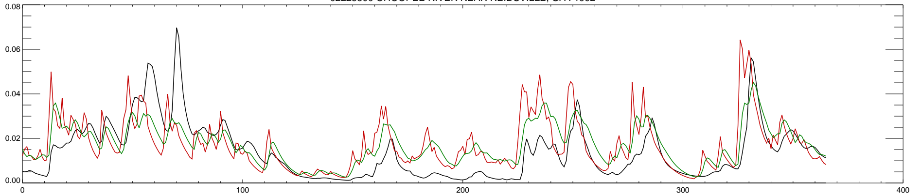
02225500 OHOOPEE RIVER NEAR REIDSVILLE, GA : 1993
