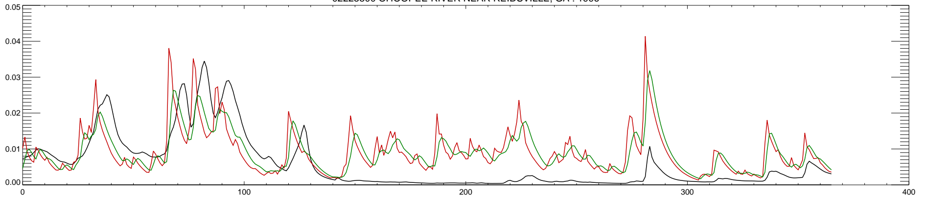
02225500 OHOOPEE RIVER NEAR REIDSVILLE, GA : 1997
