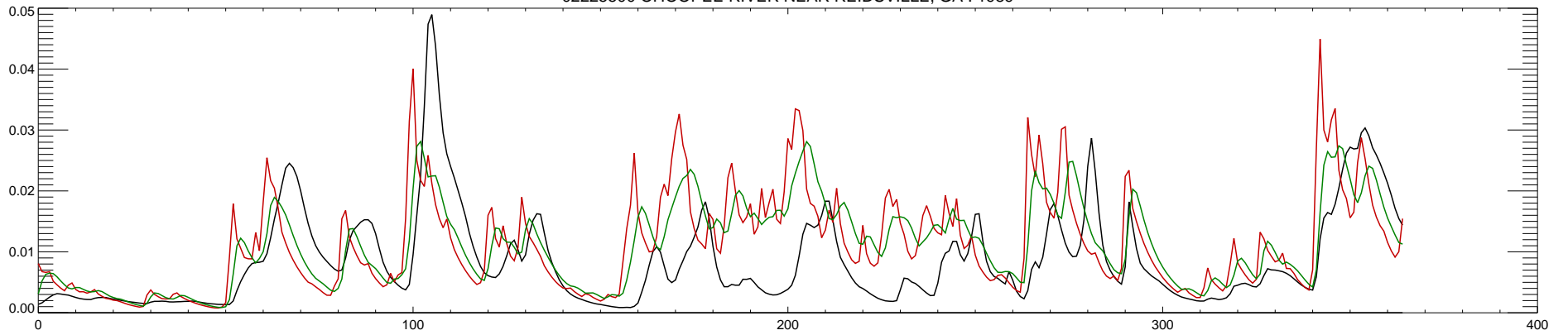
02225500 OHOOPEE RIVER NEAR REIDSVILLE, GA : 1990
