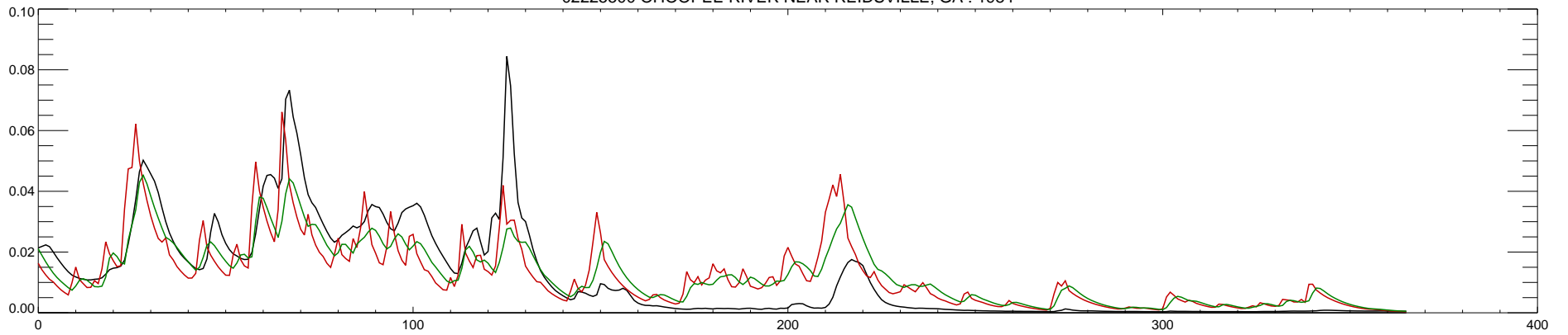
02225500 OHOOPEE RIVER NEAR REIDSVILLE, GA : 1985
