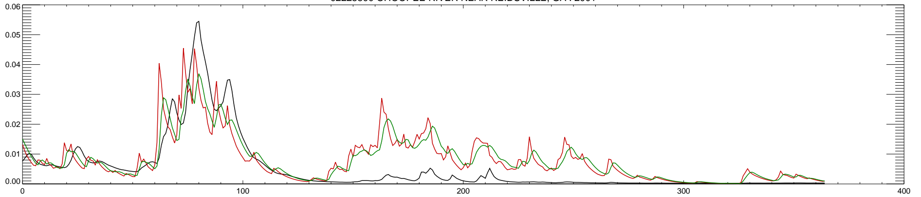
02225500 OHOOPEE RIVER NEAR REIDSVILLE, GA : 2002
