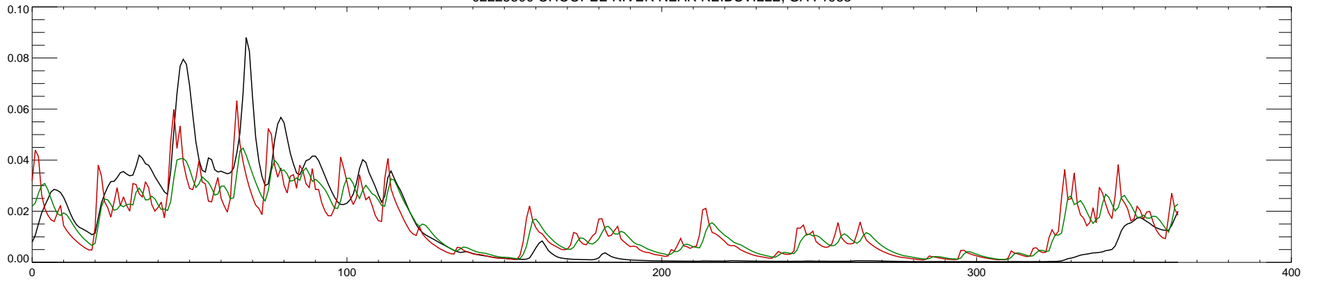
02225500 OHOOPEE RIVER NEAR REIDSVILLE, GA : 1984
