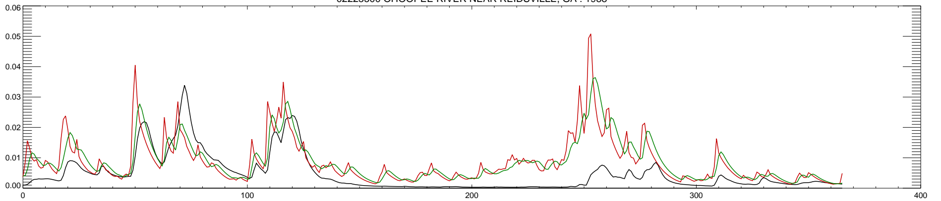
02225500 OHOOPEE RIVER NEAR REIDSVILLE, GA : 1988
