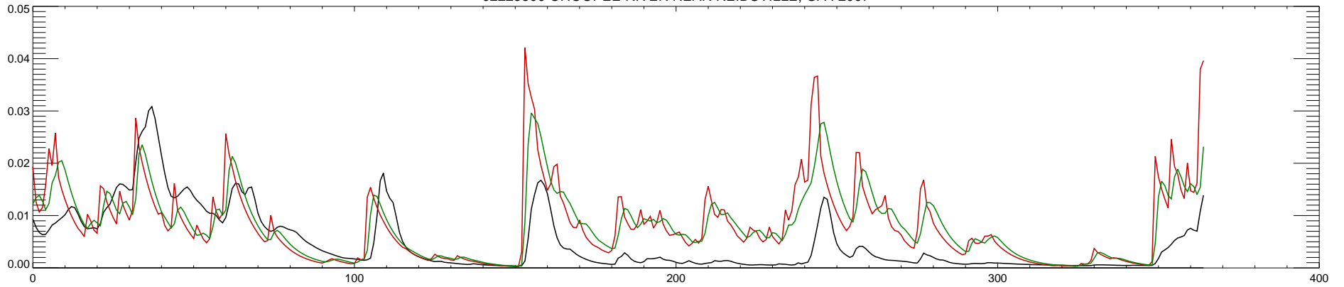
02225500 OHOOPEE RIVER NEAR REIDSVILLE, GA : 2008
