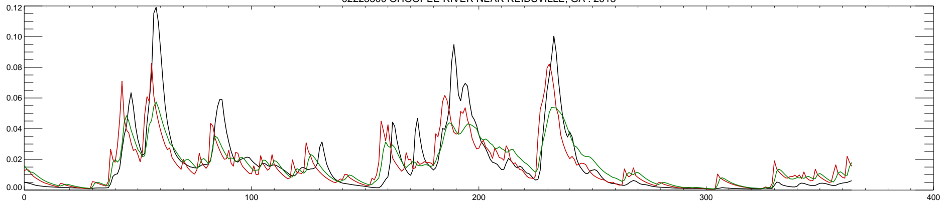
02225500 OHOOPEE RIVER NEAR REIDSVILLE, GA : 2014
