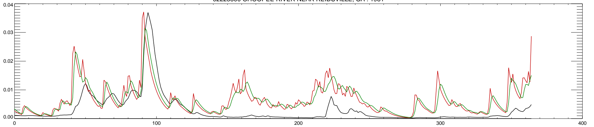
02225500 OHOOPEE RIVER NEAR REIDSVILLE, GA : 1982
