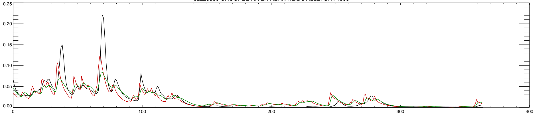
02225500 OHOOPEE RIVER NEAR REIDSVILLE, GA : 1999
