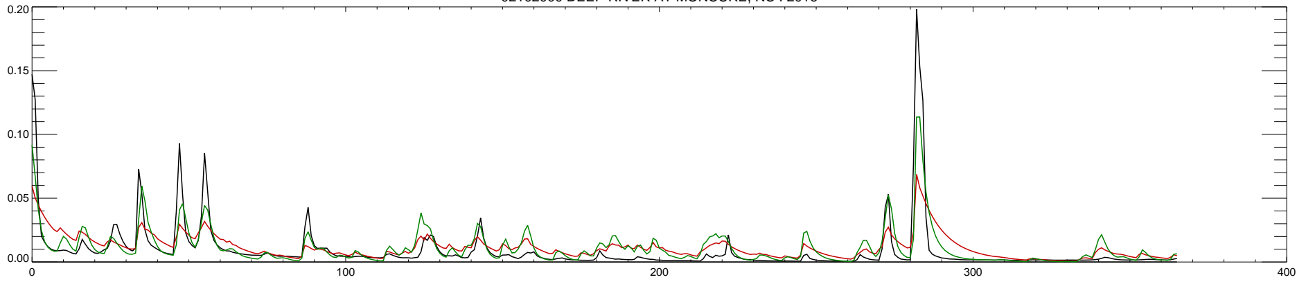
02102000 DEEP RIVER AT MONCURE, NC : 2016
