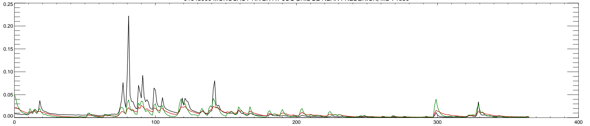
01643000 MONOCACY RIVER AT JUG BRIDGE NEAR FREDERICK, MD : 1981
