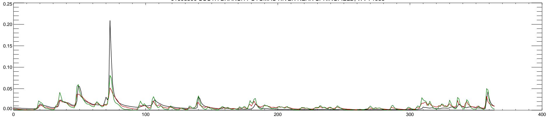
01608500 SOUTH BRANCH POTOMAC RIVER NEAR SPRINGFIELD, WV : 1987
