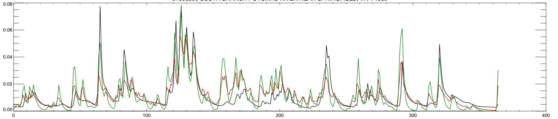
01608500 SOUTH BRANCH POTOMAC RIVER NEAR SPRINGFIELD, WV : 1990
