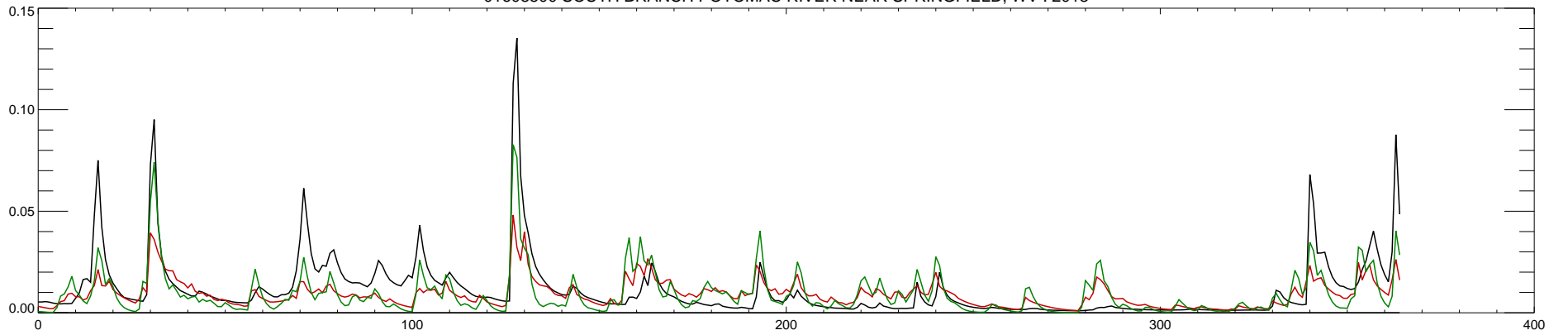
01608500 SOUTH BRANCH POTOMAC RIVER NEAR SPRINGFIELD, WV : 2014
