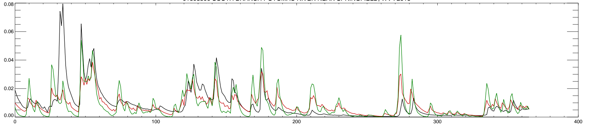
01608500 SOUTH BRANCH POTOMAC RIVER NEAR SPRINGFIELD, WV : 2016
