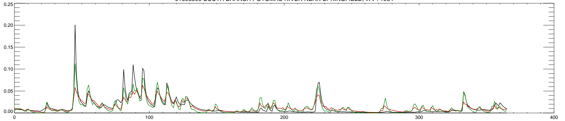
01608500 SOUTH BRANCH POTOMAC RIVER NEAR SPRINGFIELD, WV : 1985
