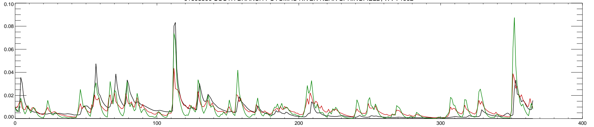
01608500 SOUTH BRANCH POTOMAC RIVER NEAR SPRINGFIELD, WV : 1993
