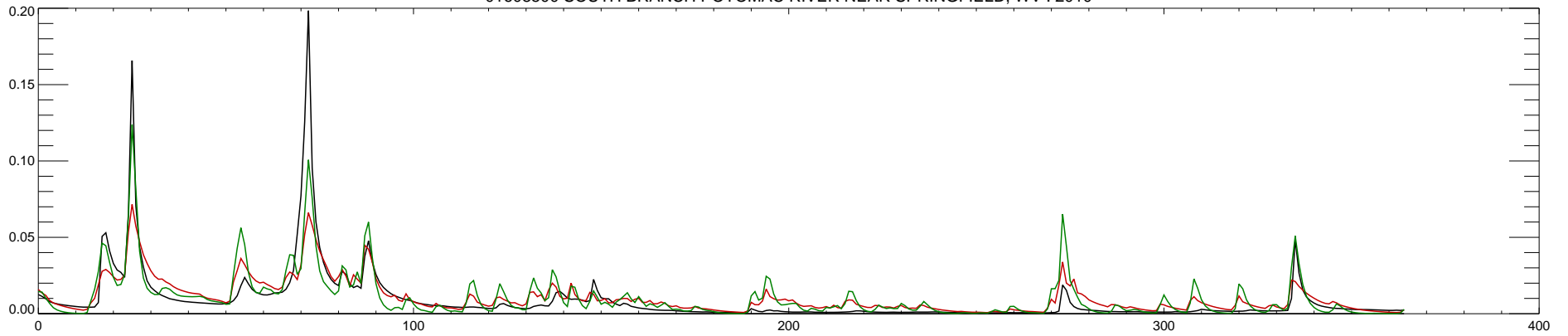
01608500 SOUTH BRANCH POTOMAC RIVER NEAR SPRINGFIELD, WV : 2011
