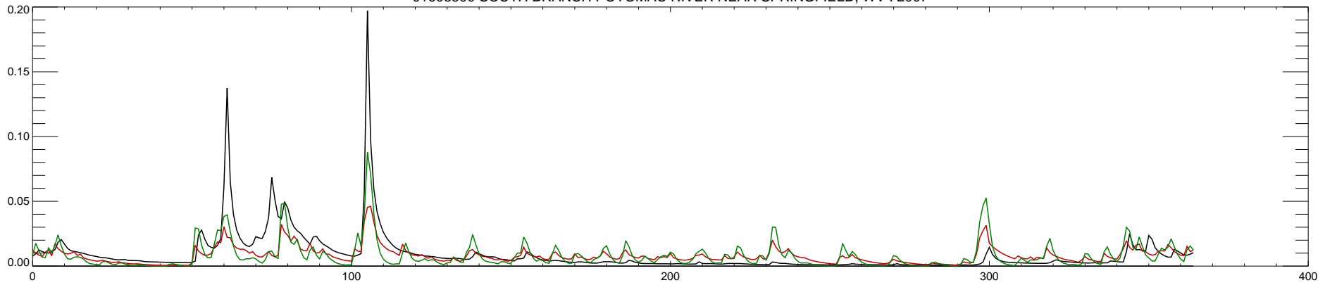
01608500 SOUTH BRANCH POTOMAC RIVER NEAR SPRINGFIELD, WV : 2008
