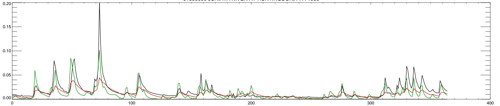
01559000 JUNIATA RIVER AT HUNTINGDON, PA : 1987
