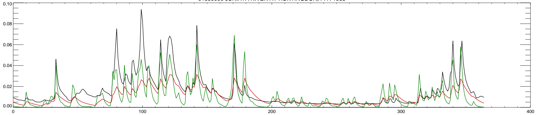
01559000 JUNIATA RIVER AT HUNTINGDON, PA : 1984
