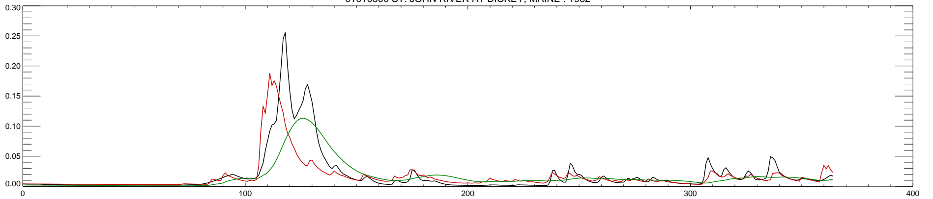
01010500 ST. JOHN RIVER AT DICKEY, MAINE : 1982
