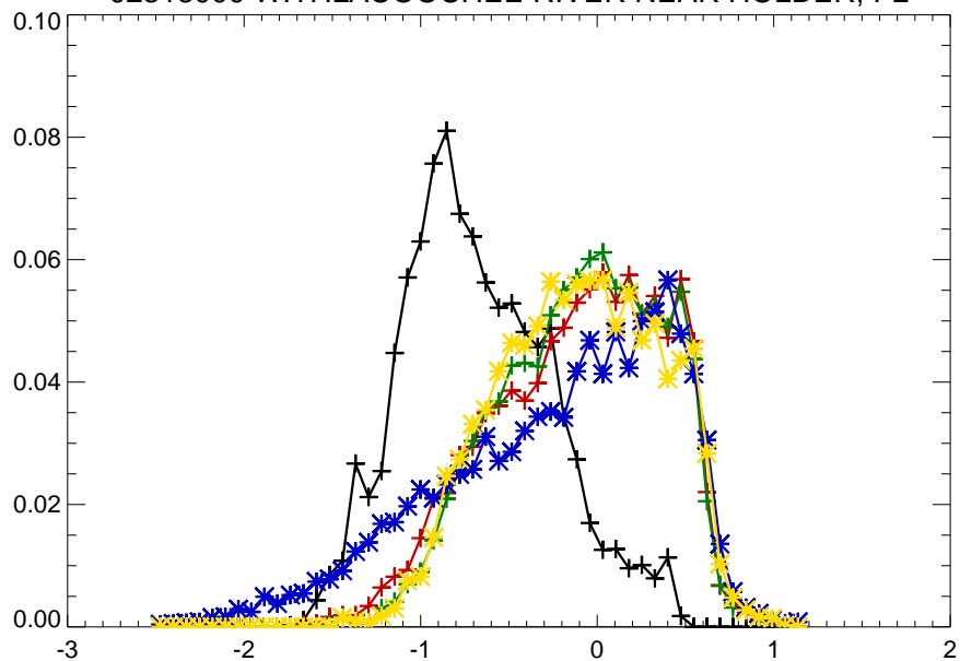
02313000 WITHLACOCHEE RIVER NEAR HOLDER, FL
