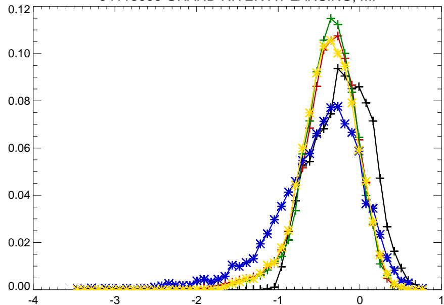
04113000 GRAND RIVER AT LANSING, MI
