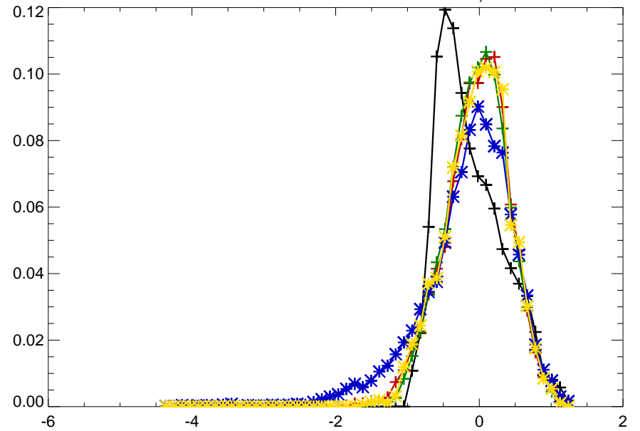
02475000 LEAF RIVER NR MCLAIN, MS
