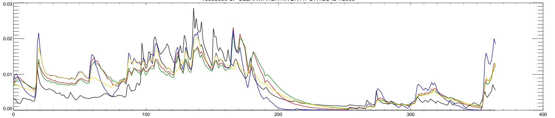
13338500 SF CLEARWATER RIVER AT STITES ID : 2006
