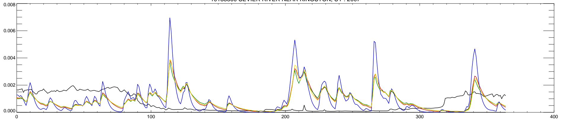
10183500 SEVIER RIVER NEAR KINGSTON, UT : 2007
