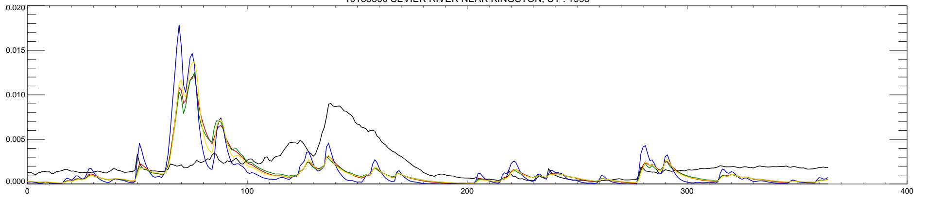
10183500 SEVIER RIVER NEAR KINGSTON, UT : 1994
