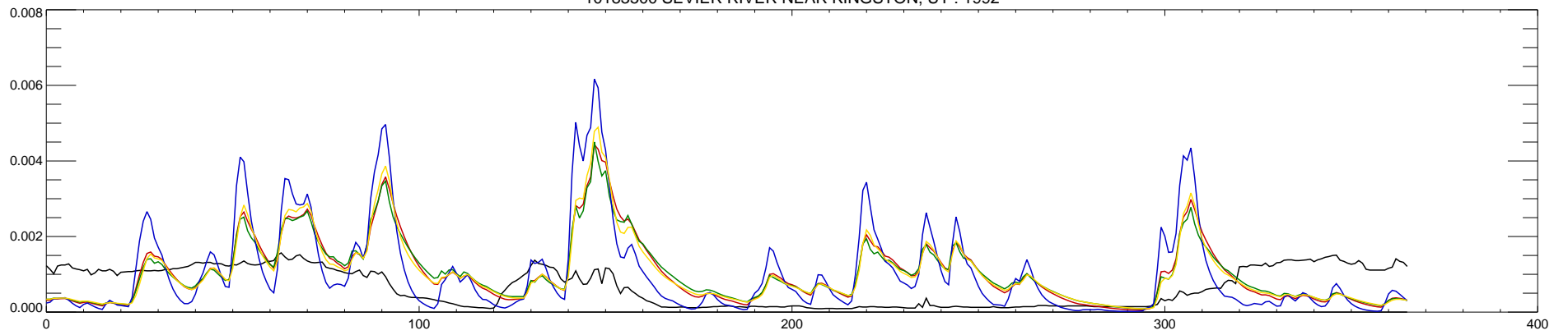
10183500 SEVIER RIVER NEAR KINGSTON, UT : 1992
