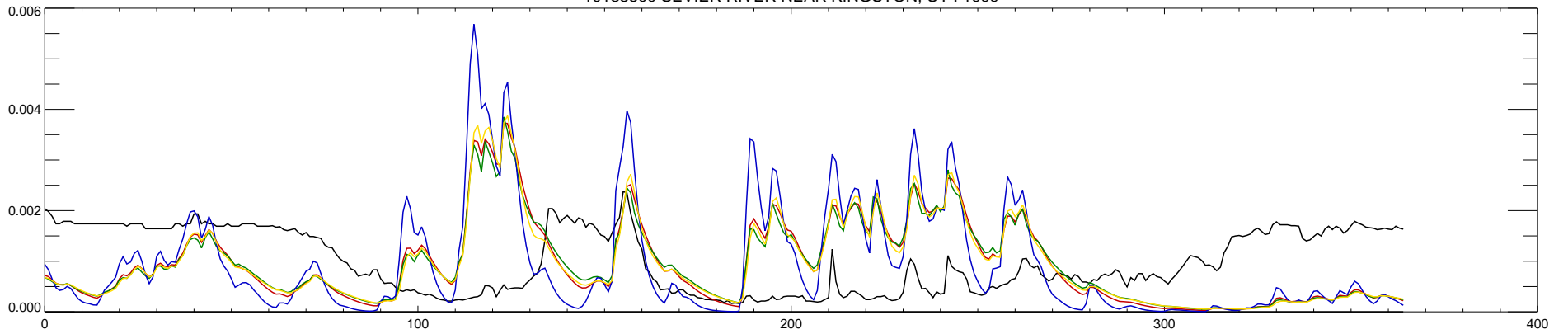
10183500 SEVIER RIVER NEAR KINGSTON, UT : 2000
