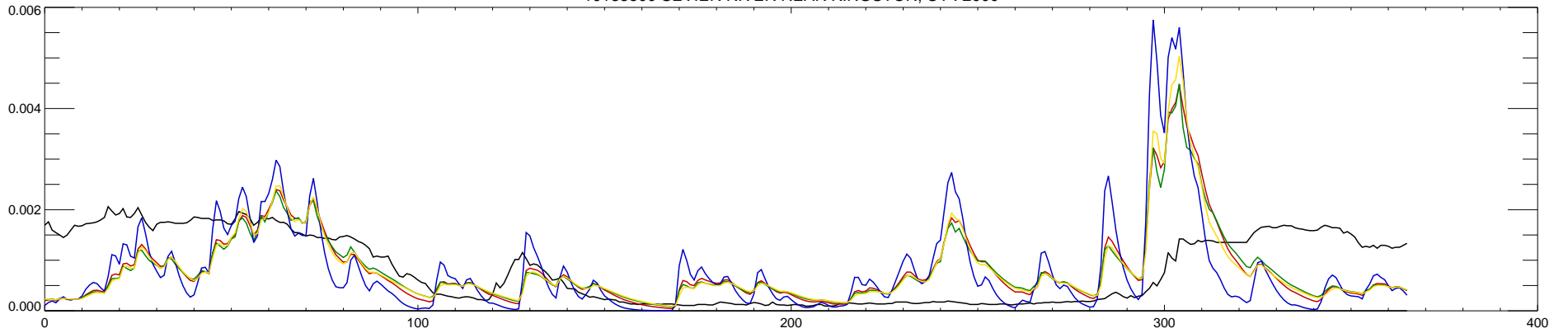
10183500 SEVIER RIVER NEAR KINGSTON, UT : 2001
