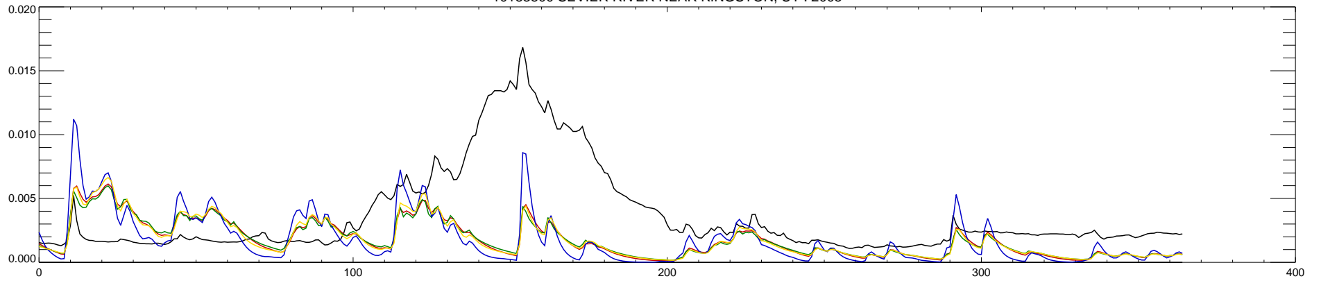
10183500 SEVIER RIVER NEAR KINGSTON, UT : 2006
