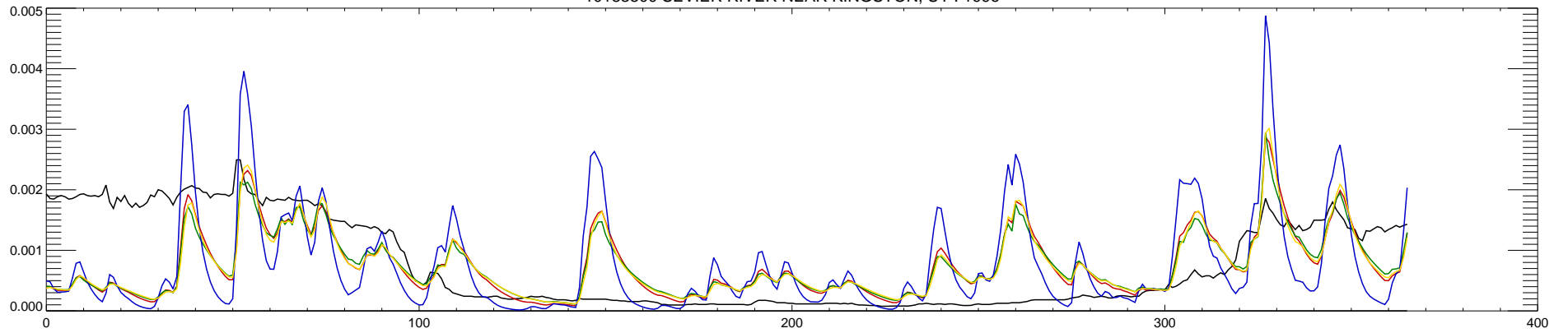
10183500 SEVIER RIVER NEAR KINGSTON, UT : 1997
