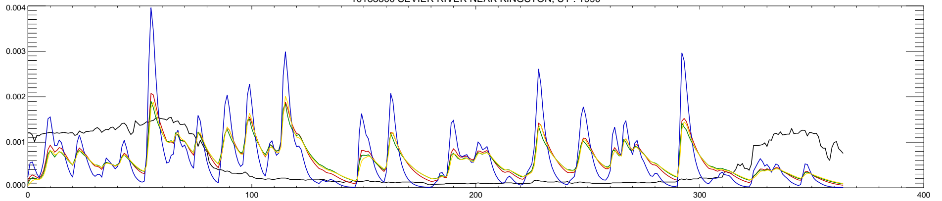
10183500 SEVIER RIVER NEAR KINGSTON, UT : 1991
