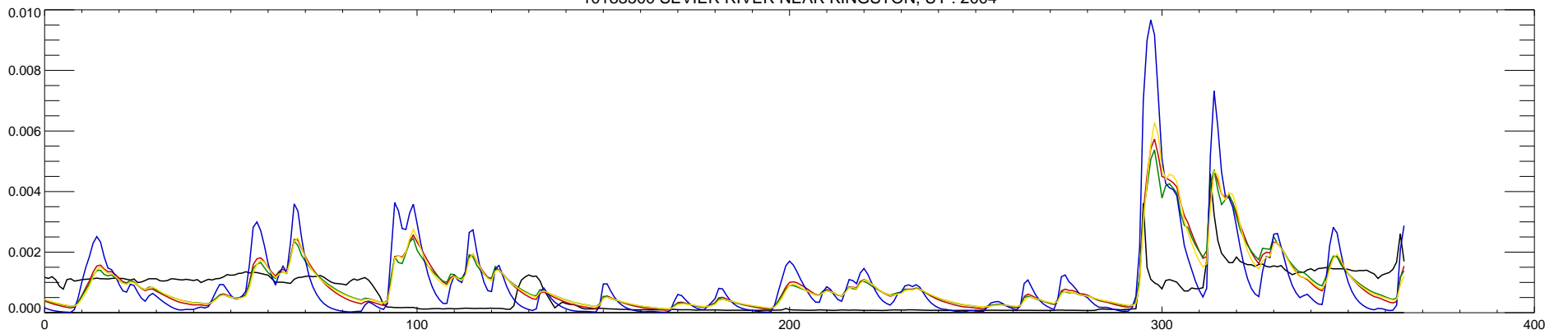
10183500 SEVIER RIVER NEAR KINGSTON, UT : 2004
