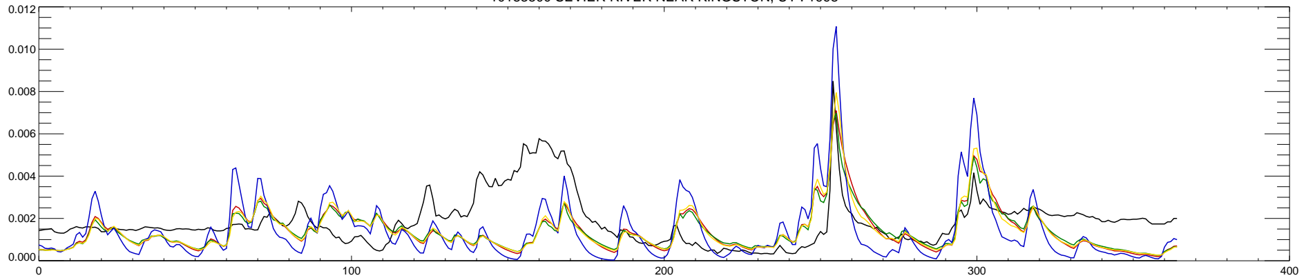
10183500 SEVIER RIVER NEAR KINGSTON, UT : 1998
