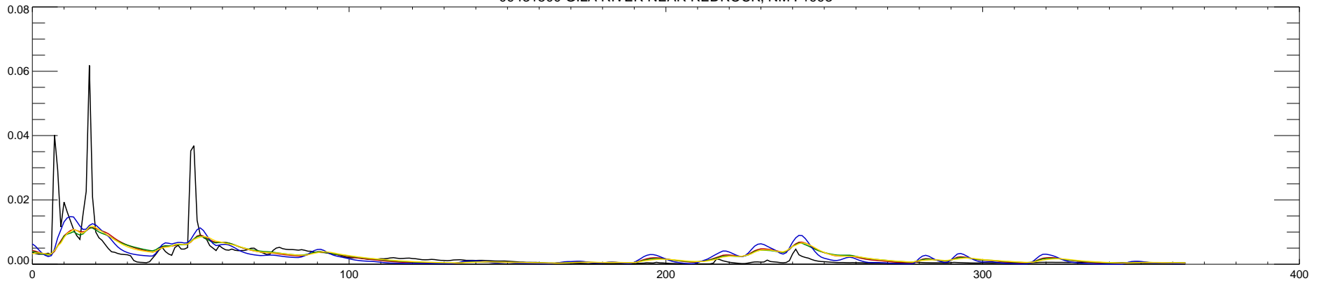
09431500 GILA RIVER NEAR REDROCK, NM : 1994
