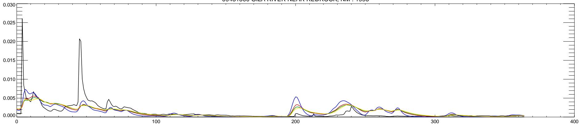
09431500 GILA RIVER NEAR REDROCK, NM : 1995
