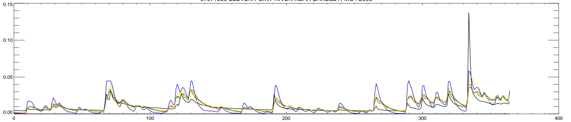
07071500 ELEVEN POINT RIVER NEAR BARDLEY, MO : 2007
