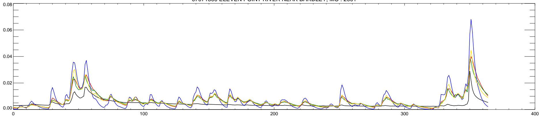
07071500 ELEVEN POINT RIVER NEAR BARDLEY, MO : 2001
