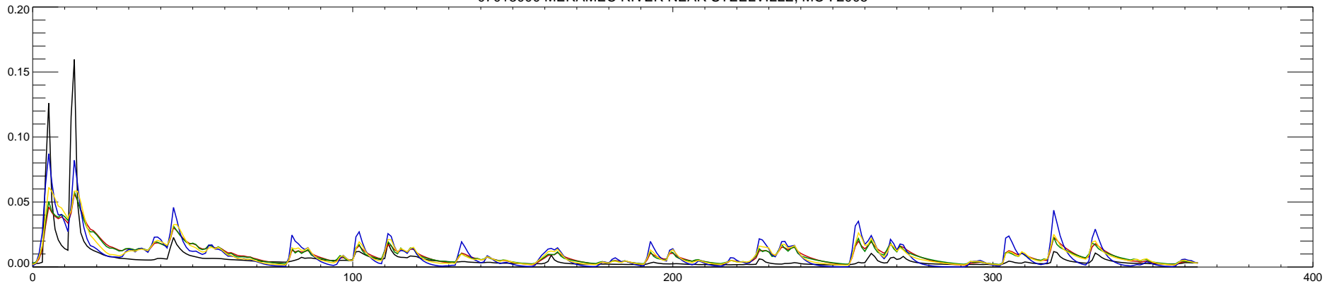
07013000 MERAMEC RIVER NEAR STEELVILLE, MO : 2006
