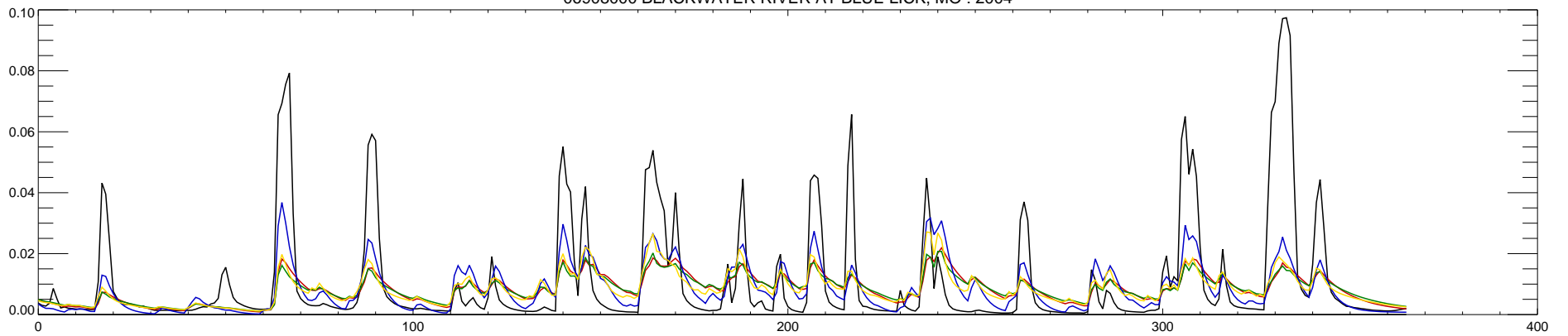
06908000 BLACKWATER RIVER AT BLUE LICK, MO : 2004
