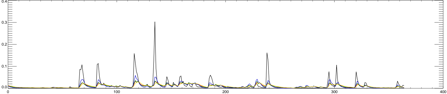
06899500 THOMPSON RIVER AT TRENTON, MO : 2009
