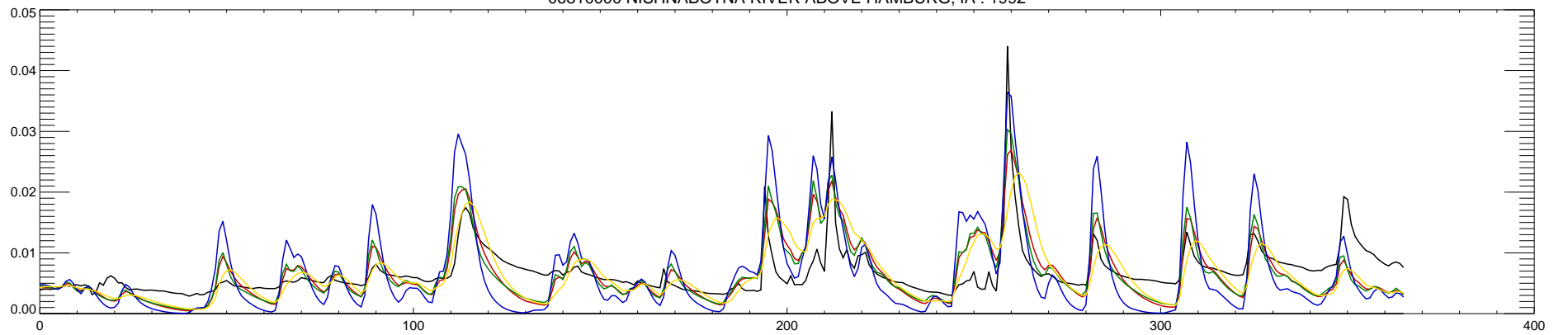
06810000 NISHNABOTNA RIVER ABOVE HAMBURG, IA : 1992
