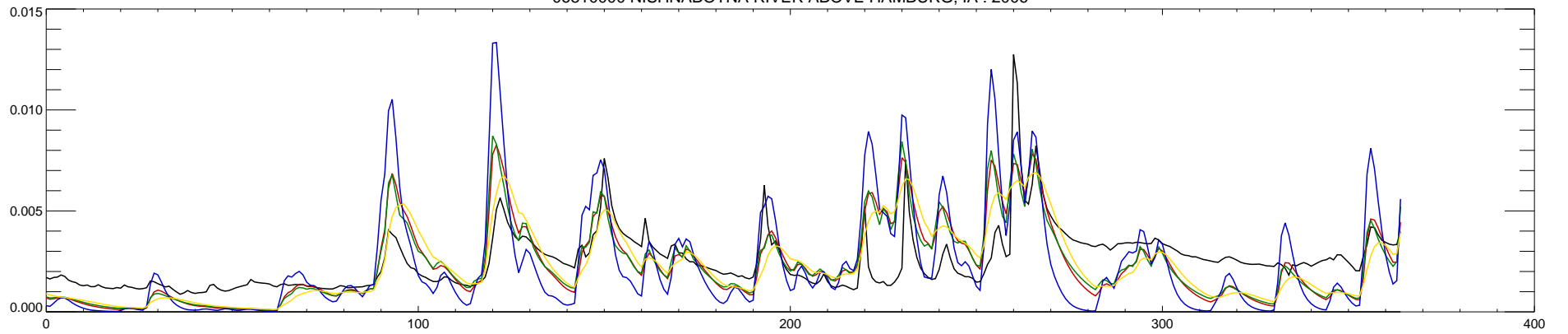
06810000 NISHNABOTNA RIVER ABOVE HAMBURG, IA : 2007
