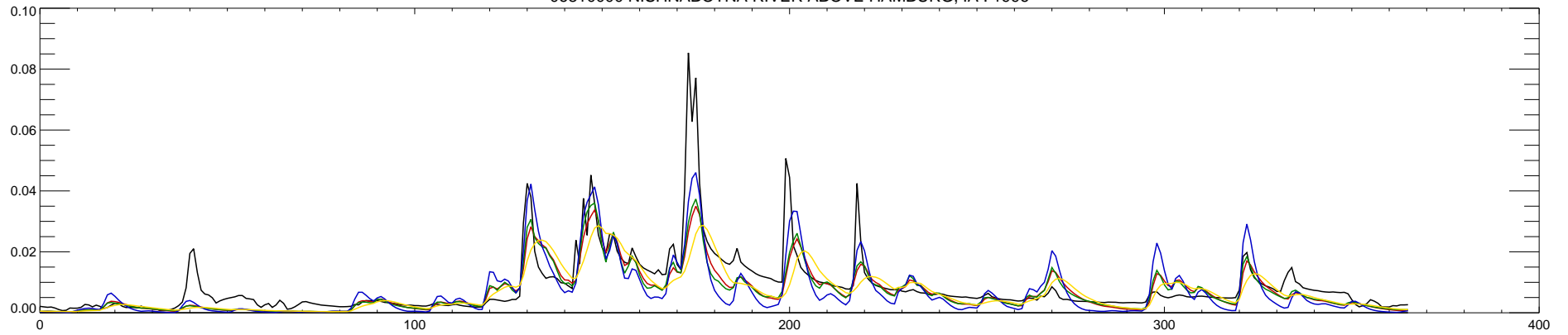
06810000 NISHNABOTNA RIVER ABOVE HAMBURG, IA : 1997
