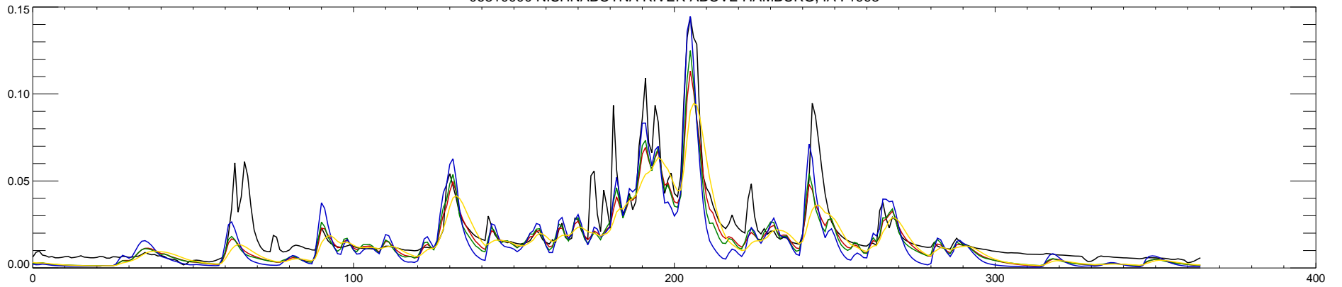
06810000 NISHNABOTNA RIVER ABOVE HAMBURG, IA : 1994
