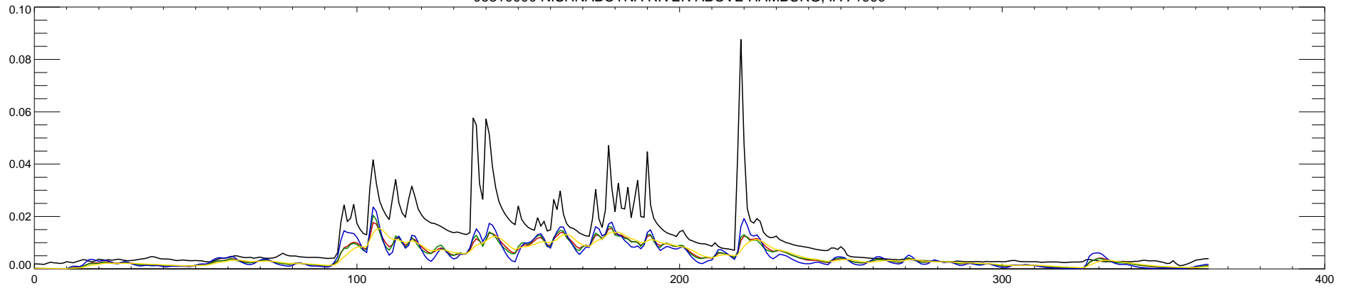
06810000 NISHNABOTNA RIVER ABOVE HAMBURG, IA : 2000
