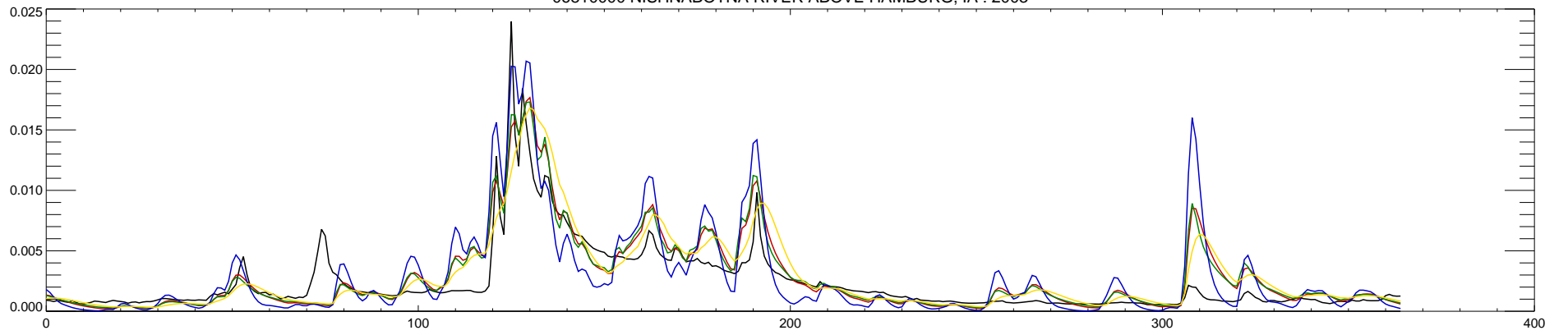
06810000 NISHNABOTNA RIVER ABOVE HAMBURG, IA : 2004
