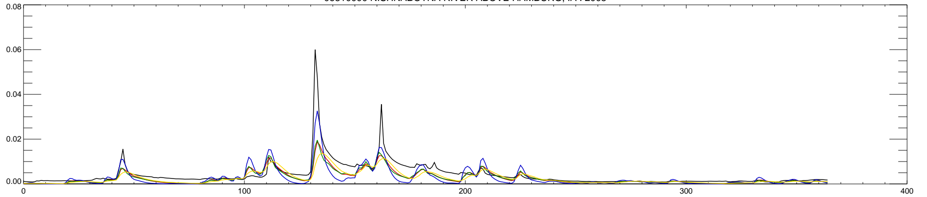
06810000 NISHNABOTNA RIVER ABOVE HAMBURG, IA : 2006
