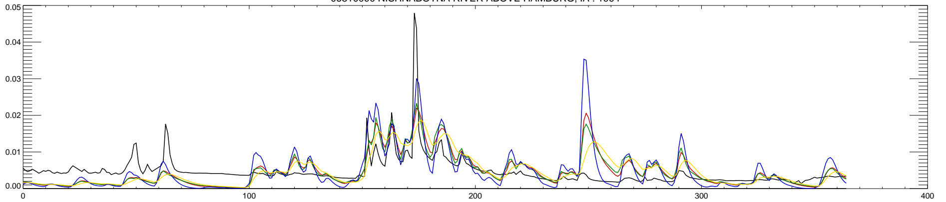
06810000 NISHNABOTNA RIVER ABOVE HAMBURG, IA : 1995
