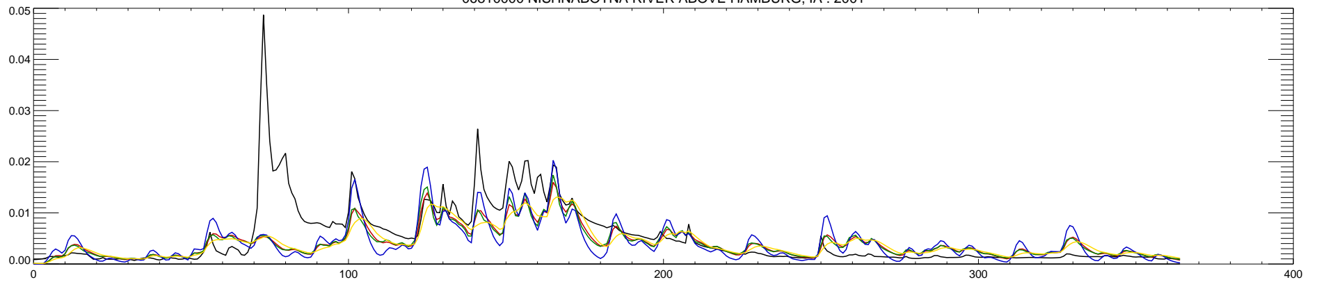
06810000 NISHNABOTNA RIVER ABOVE HAMBURG, IA : 2001
