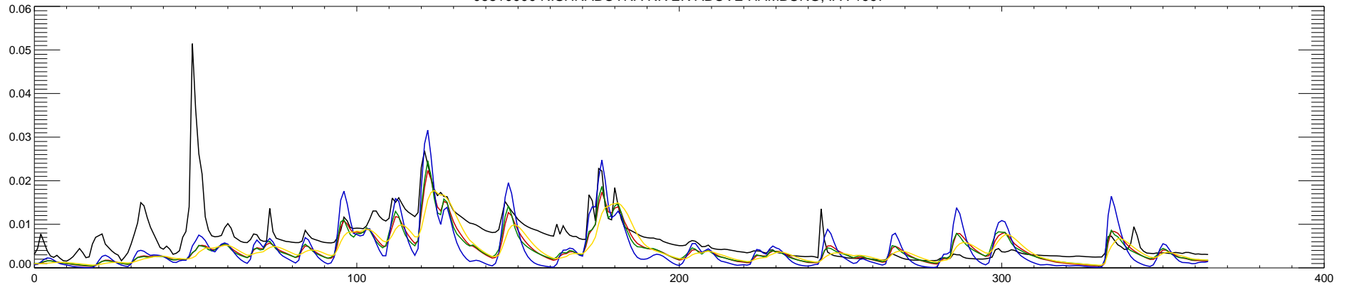
06810000 NISHNABOTNA RIVER ABOVE HAMBURG, IA : 1998
