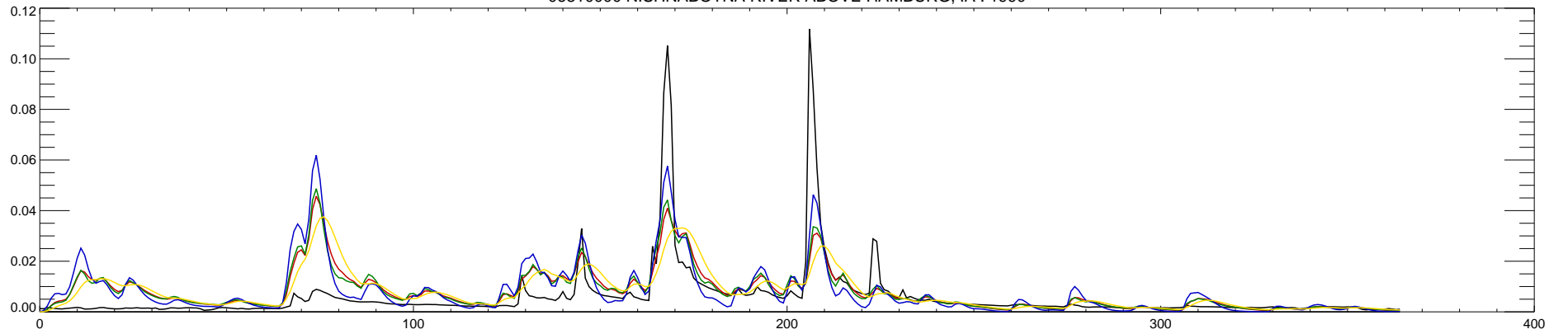
06810000 NISHNABOTNA RIVER ABOVE HAMBURG, IA : 1991
