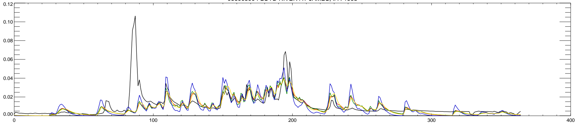
06600500 FLOYD RIVER AT JAMES, IA : 1994
