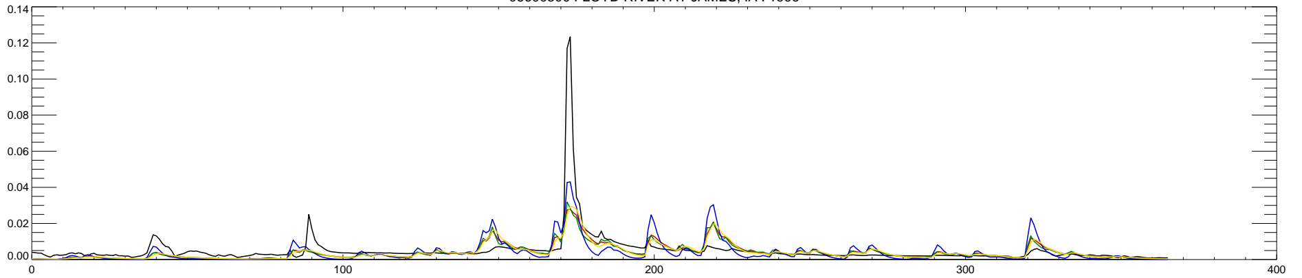
06600500 FLOYD RIVER AT JAMES, IA : 1997
